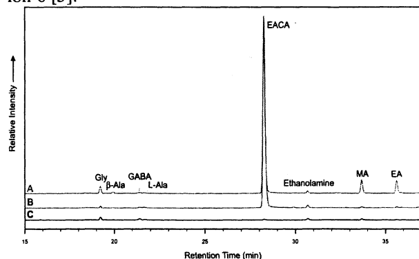
Figure 1. Fluorescence chromatograms from the liquid chromatography-fluorescence detection-time of flight mass spectrometry analyses showing amines detected in: A , Stardust comet-exposed aerogel; B , Stardust aerogel witness tile (not comet-exposed); and C , un-flown aerogel (figure adapted from [6]).
