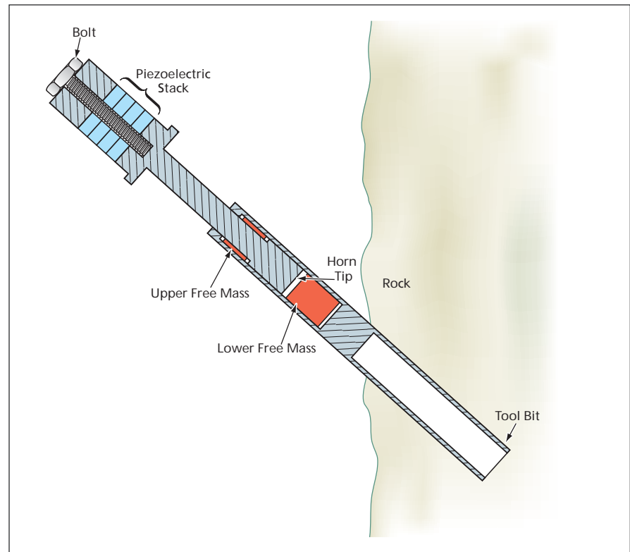
The Ultrasonic/Sonic Anchor drills its own anchor hole in a rock face.
