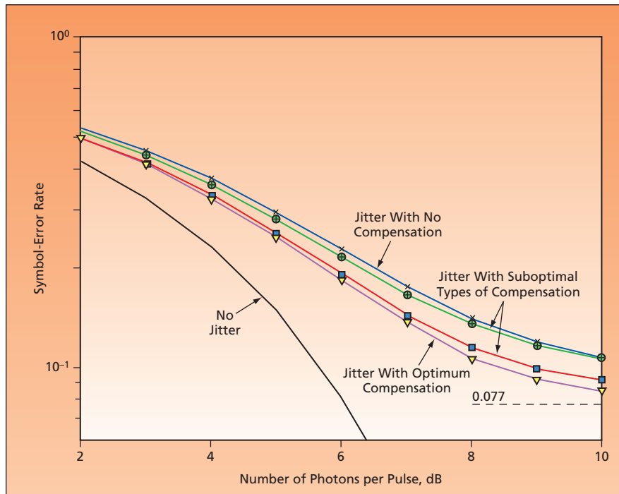
Symbol-Error Rates were computed for a PPM receiver not subject to jitter and for PPM receivers subject to photon-arrival-jitter-induced inter-time-slot interference (neglecting inter-symbol interference), all for the case of 16-time-slot PPM words with an average of 0.2 noise photons per time slot and \alpha = 0.2 in a jitter-offset exponential distribution f(\delta) = [1/(2\alpha)]e^{-\delta/\alpha} , where \delta is the jitter offset in units of one slot duration.
