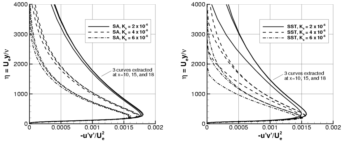
Figure 15. Turbulent shear stress profiles for SA and SST for 2-D sink-flow at three different streamwise acceleration parameters.
