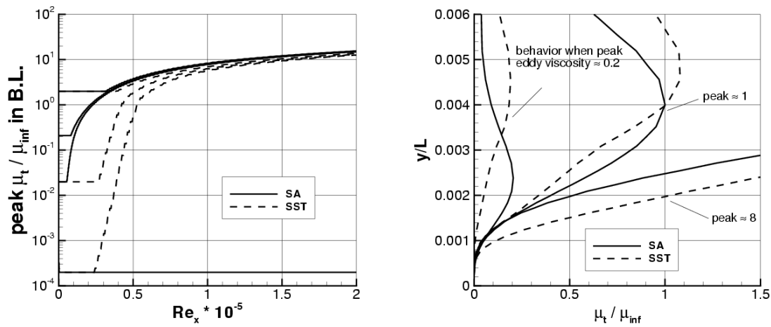
Figure 8. Eddy viscosity over flat plate, M = 0.2 , medium grid; (a) peak value for various freestream turbulence levels; (b) vertical profile at locations where peak \mu_t / \mu_{\infty} \approx 0.2, 1.0, \text{ and } 8.0 .
