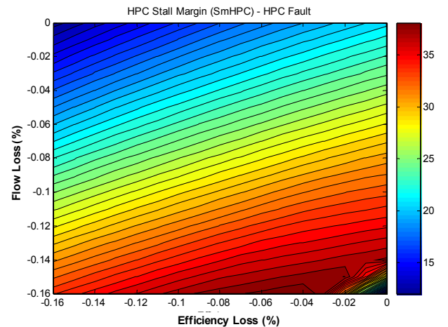
Figure 3. Response surface of HPC stall margin as a function of efficiency and flow losses simulating degradation in HPC module
