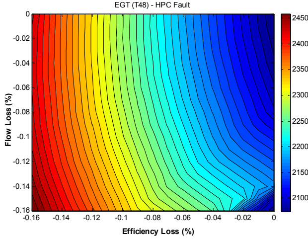
Figure 4. Response surface for Exhaust Gas Temperature (EGT) as a function of efficiency and flow losses
