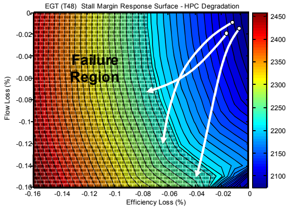
Figure 8. Fault propagation trajectories on EGT contour map with failure threshold
