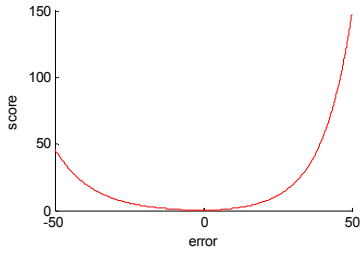
Figure 9. Score as a function of error
