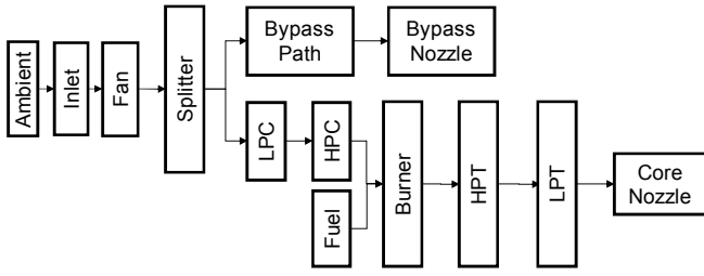
Figure 2. A layout showing various modules and their connections as modeled in the simulation [9]
