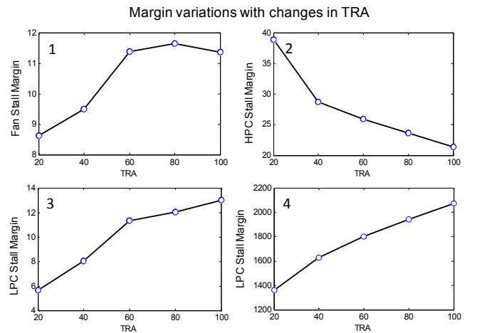
Figure 6. Stall margins vary as a function of operational conditions (TRA in this example)
