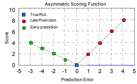
Figure 11. A simplified asymmetric scoring function chosen for illustration
