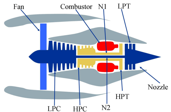
Figure 1. Simplified diagram of engine simulated in C-MAPSS [9]
