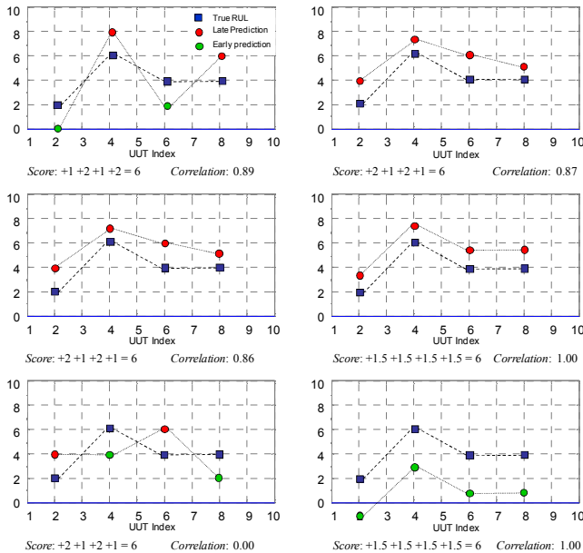
Figure 10. Scenarios illustrating various cases where error based scores may be same but the correlation score distinguishes further between different algorithms
