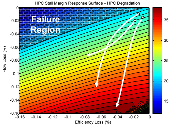
Figure 7. Fault propagation trajectories on HPC stall margin contour map
