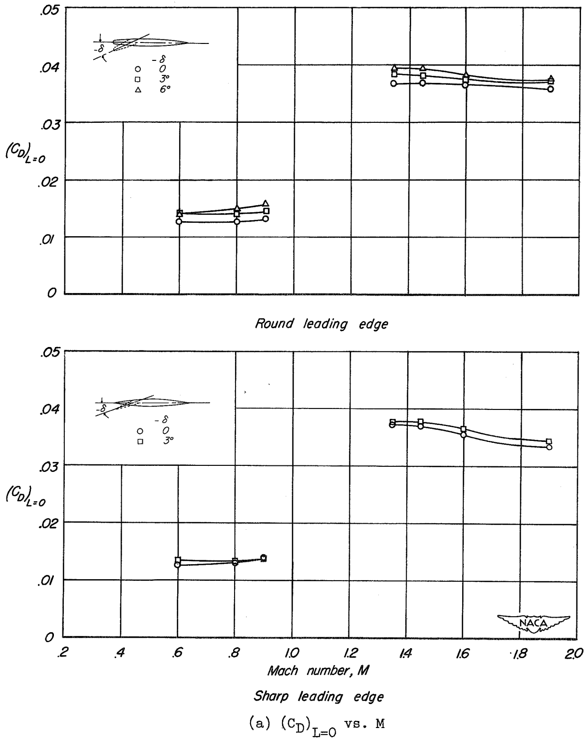
Figure 4.- Effect of flap deflection upon the variation with Mach number of the drag at zero lift and maximum lift-drag ratio of each model; R=3.0 million.
