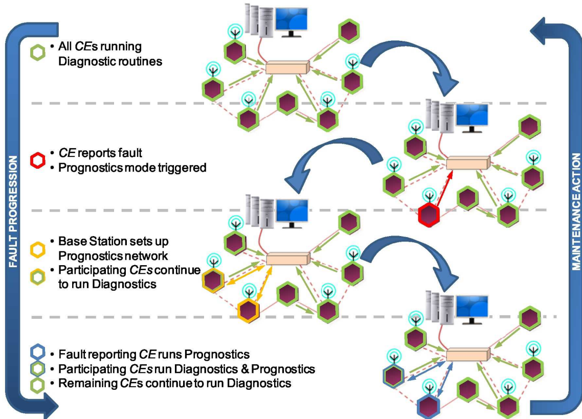
Figure 2 – Flow diagram for diagnostics and prognostics operations in the distributed architecture.
