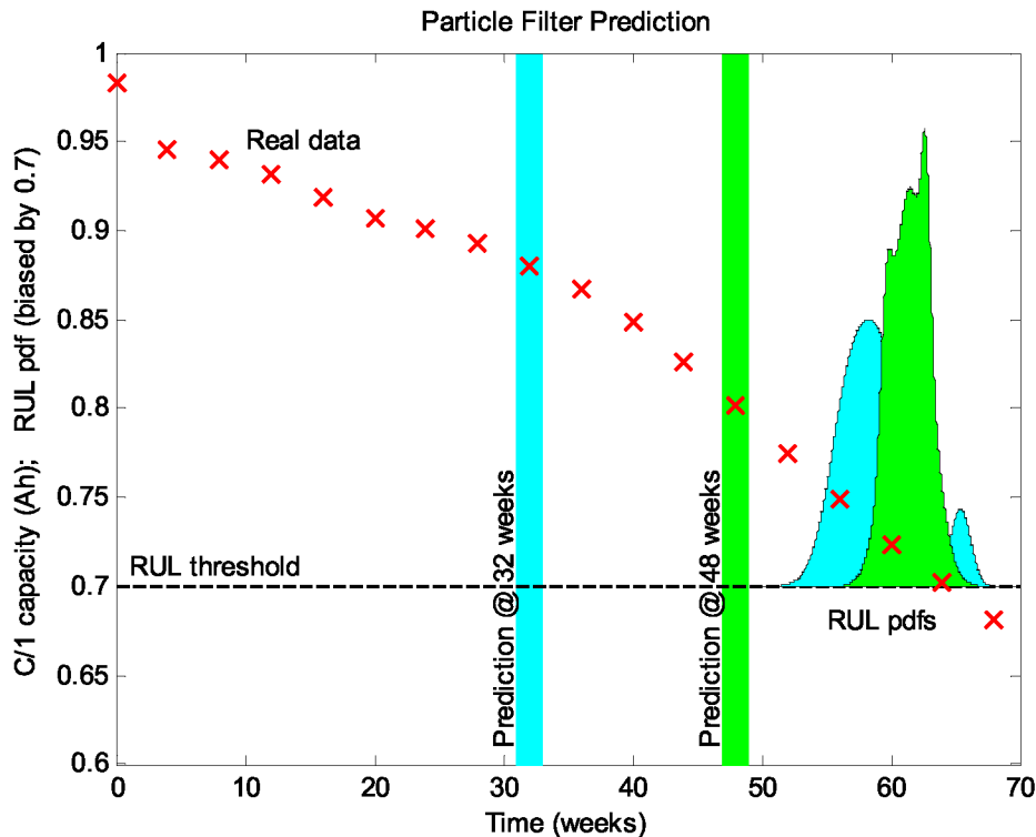
Figure 7 – Distributed PF prediction at 32 and 48 weeks.
