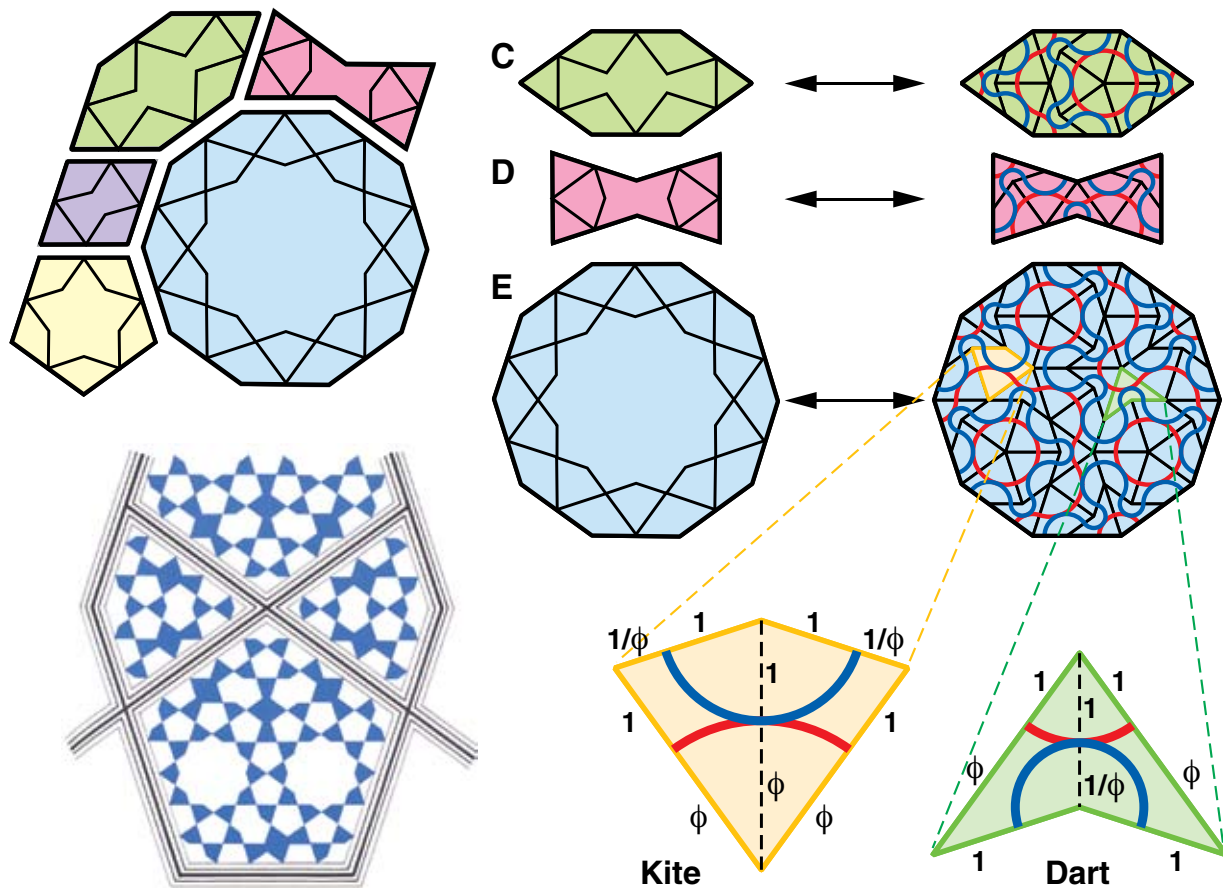
Figure 5-18. The five basic girih tile shapes (decagon, pentagon, rhombus, hexagon, and bowtie) described in Lu & Steinhardt (2007), and Penrose's darts and kites.
