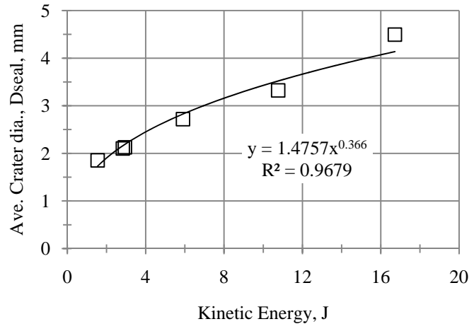
Figure 8. Average Crater Surface Diameter in Parker 0S383-70 from Projectiles of Different Kinetic Energy. Hits more than 25% of the seal width away from the center-line, and hits at low temperatures omitted. Data included is shown in gray in Table 3. These data yield D_{seal} = 1.476KE^{0.366} .
