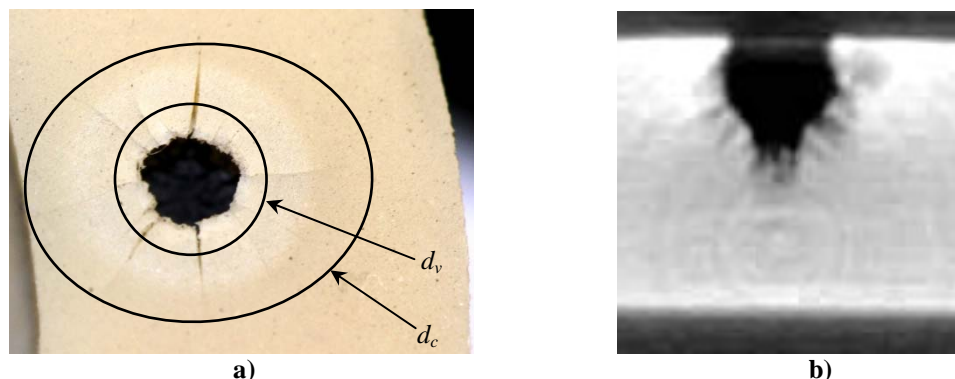
Figure 4. Cratered Esterline seal. a) Top view of the 9.1 mm wide Esterline seal damaged by a 0.8 mm diameter, 0.728 mg Al sphere at 8.3 km/s, Strike 1; the black ellipses show d_c - the extent of cracks radiating from the crater, and d_v - the diameter of the vaporized material; b) Cross sectional view of the crater using computed tomography, seal is 5.5 mm thick, Strike 1.
