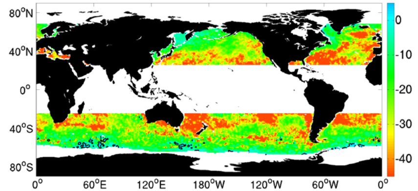
\lambda_{QLHF} , SEAFUX
