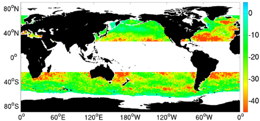
\lambda_{QLHF} , HOAPS3
