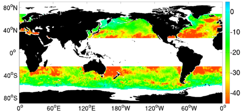
\lambda_{QLHF} , OAFUX
