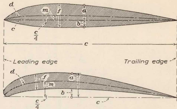
a/c, upper camber b/c, lower camber m/c, mean camber c, chord length d, mean line of the airfoil profile c/4, aerodynamic center (quarter-chord point) f, profile thickness
