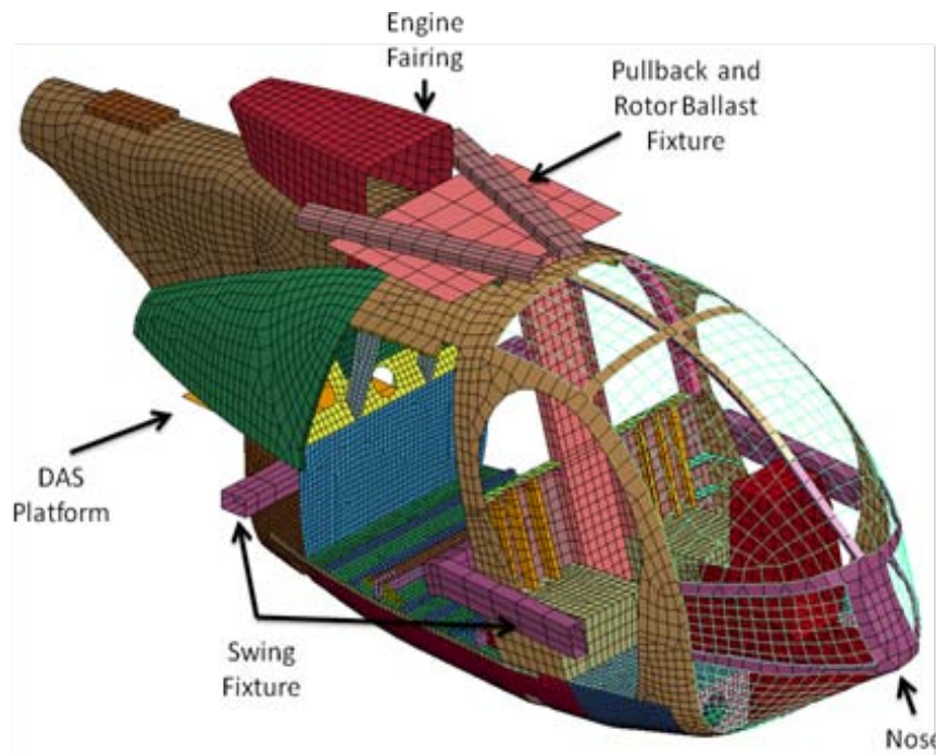
Figure 11. MD-500 Fuselage FEM
