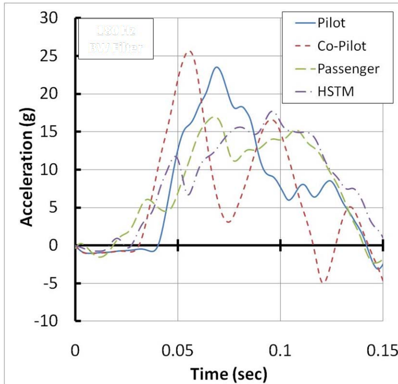
Figure 17. Pre-Test, ATD Vertical Pelvic Accelerations
