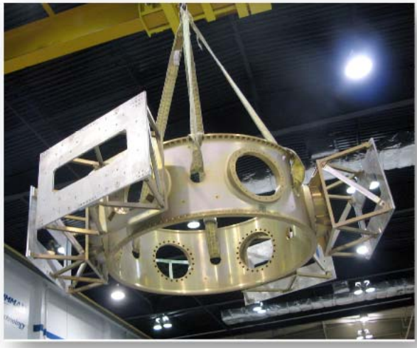
Figure 7: LCROSS ESPA Ring and Secondary Panels
