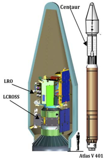
Figure 2: The LRO/LCROSS Launch Vehicle Stack
