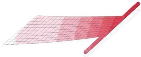
Fig. 12a. Splined mode 1.
