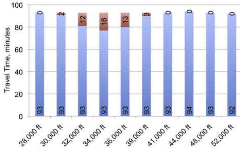
Figure 4. Travel time for the wind-optimal routes from ORD to EWR and length of periods favorable to persistent contrails formation at 10 different altitudes.
