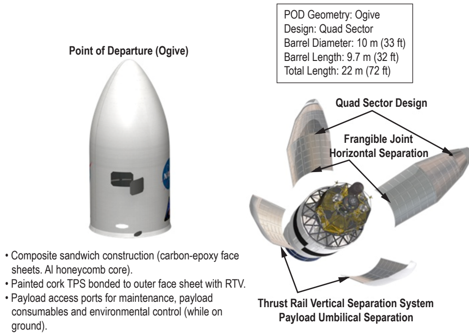
Figure 20. Ares V shroud element view.
