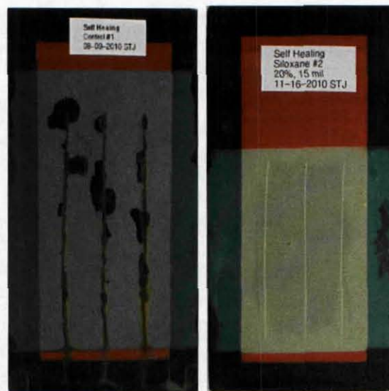
Figure 2. 700 hours of salt fog testing results of carbon steel panels coated with a control coating system (left panel) and the same coating with a siloxane healing system (right panel).
