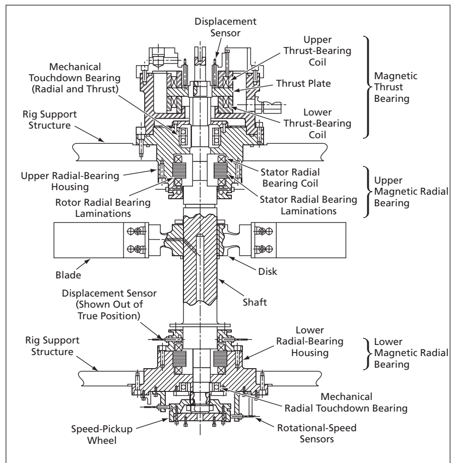
The Five-Axis, Three-Magnetic-Bearing configuration of this dynamic spin rig makes it possible to excite high-order vibrational modes of the disk-and-blade assembly. The five axes are the vertical thrust axis of the thrust bearing and two mutually perpendicular horizontal force axes for each of the two radial bearings.
