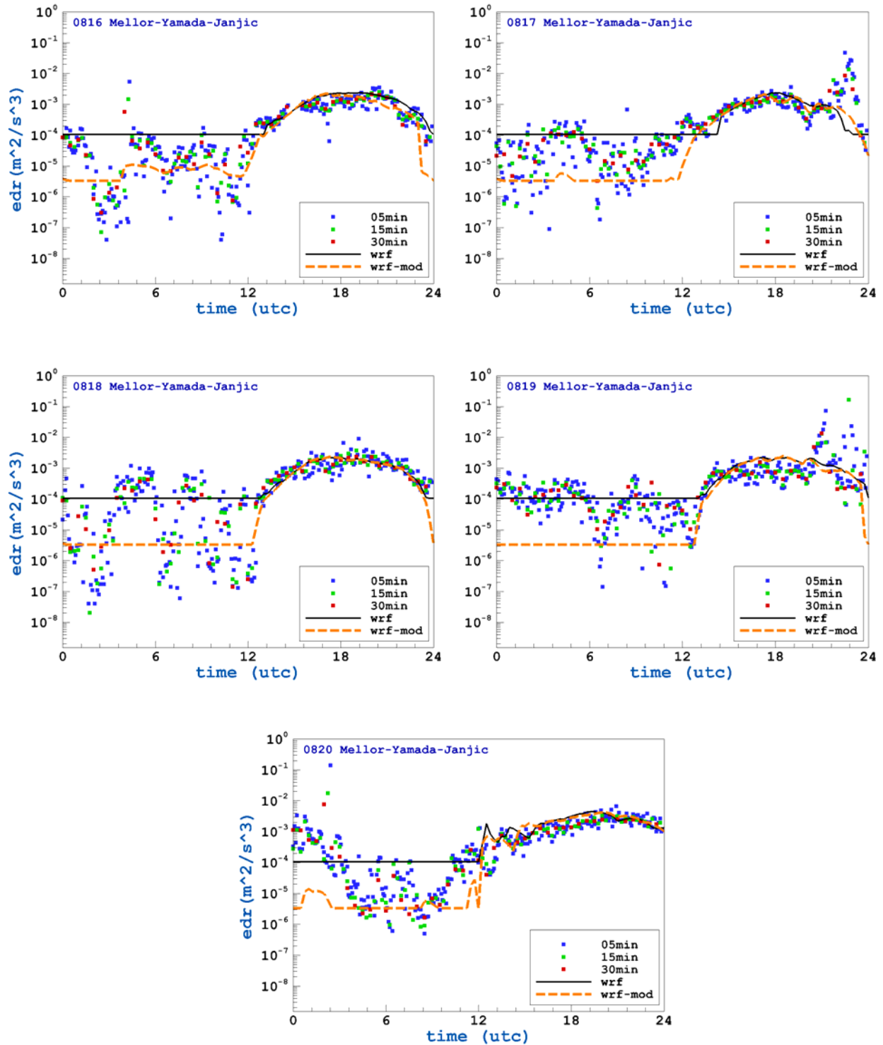
Figure 14. Comparison of simulated EDR values with observed data. Simulation results using the Mellor-Yamada-Janjic (MYJ) PBL scheme are shown for different dates. Points represent observations taken within three different time windows (5min, 15min and 30min). WRF computations are given by lines. \Delta z=40m .
