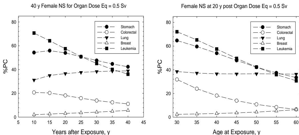
Figure 5. Calculations of %PC for NS Females for organ dose equivalents of 0.5 Sv. The left panel shows results versus time after exposure and the right panel versus age at exposure for disease diagnosis at 20 y post-exposure.
