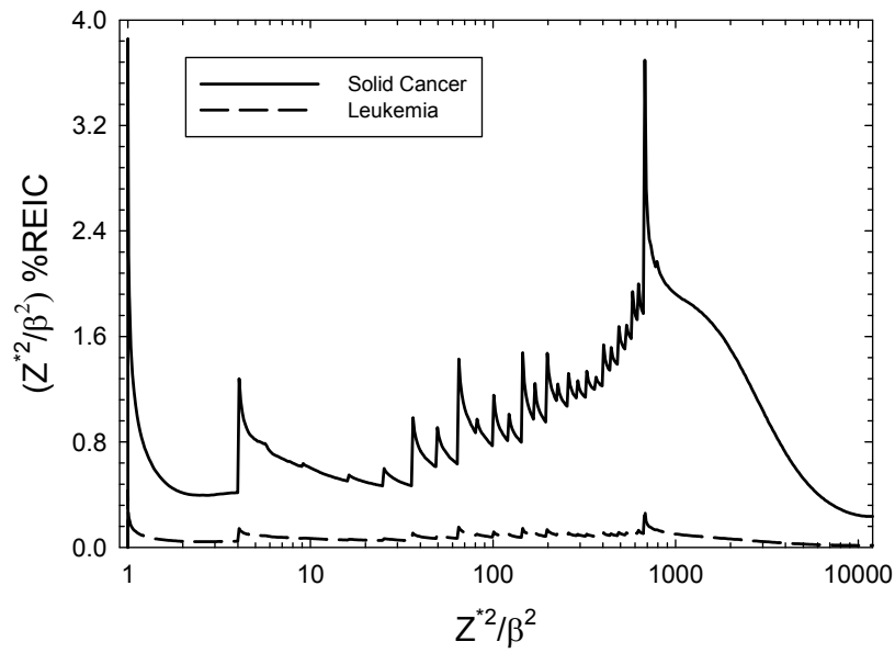
Figure 3b. Leukemia and solid cancer risk distribution for 40-y Females versus Z^2/\beta^2 for 30-month Mars mission including 18 month surface stay at solar minimum with 20 \text{ g/cm}^2 of aluminum shielding.
