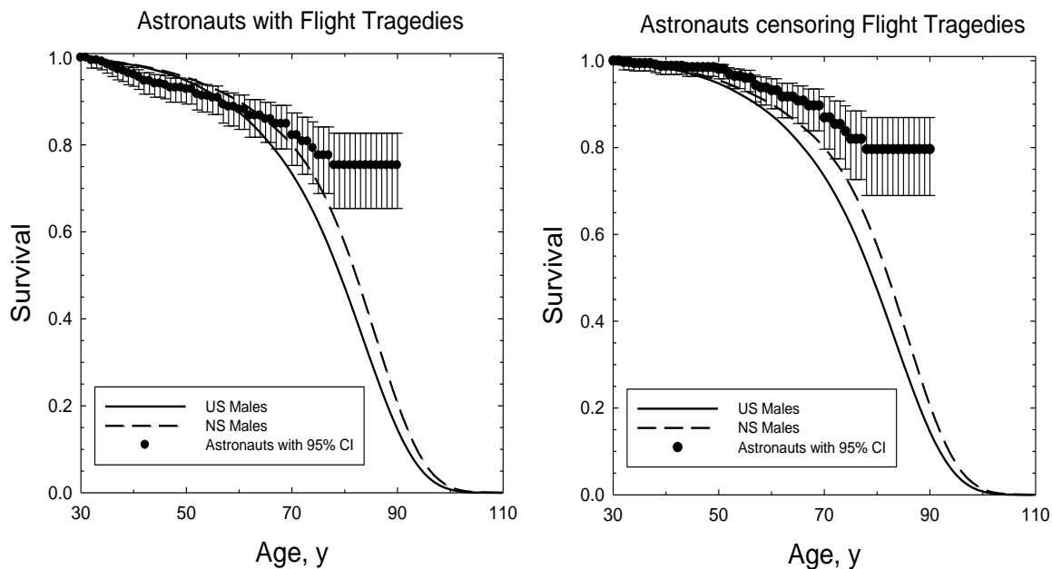
Figure 1. Kaplan-Meier survival versus age for astronauts and payload specialists compared to U.S. males and our projections for NS males. The left panel includes occupational deaths related to flight accidents or training, and right panel censors occupational deaths. Data from the Astronaut Fact Book (NASA 2005) and http://www.jsc.nasa.gov/Bios/ .
