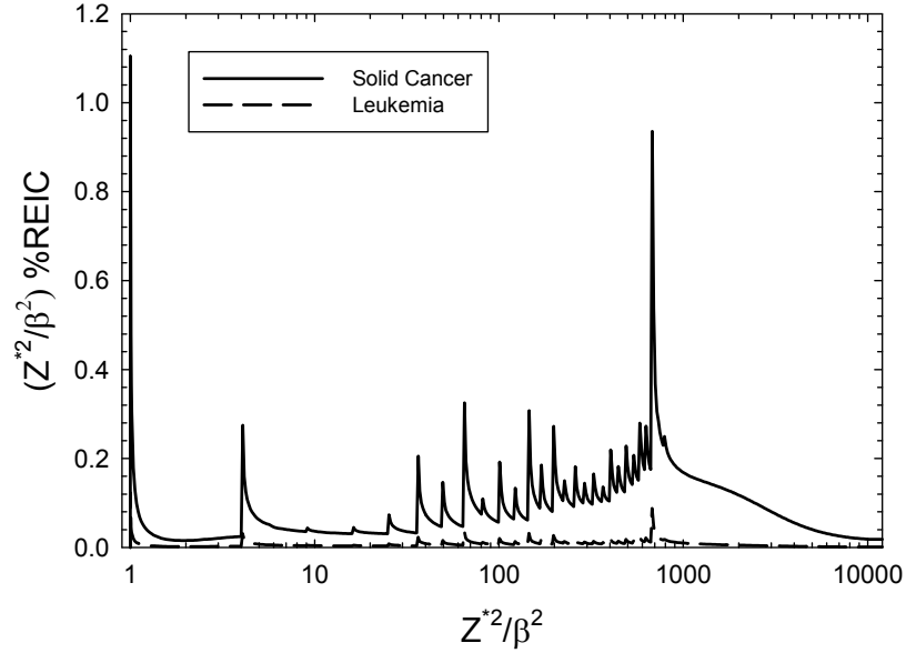
Figure 3a. Leukemia and solid cancer risk distribution for 40-y Females versus Z^2/\beta^2 on 6-month ISS mission at solar minimum with 20 \text{ g/cm}^2 of aluminum shielding.
