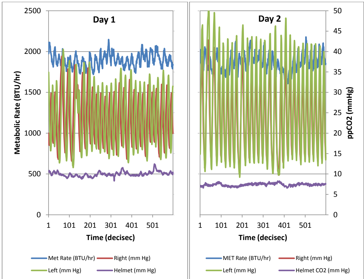
Figure 8. Example comparison of a test subject at the 2000 BTU/hr / 5 ACFM test points during the REI-suit test.
