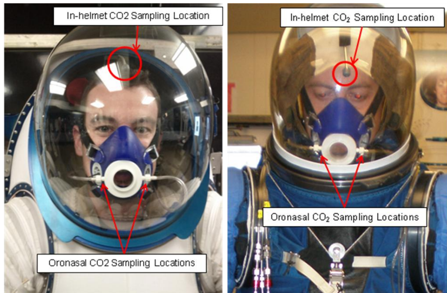
Figure 5. CO 2 sampling locations in the REI-suit (left) and EM-ACES (right).
