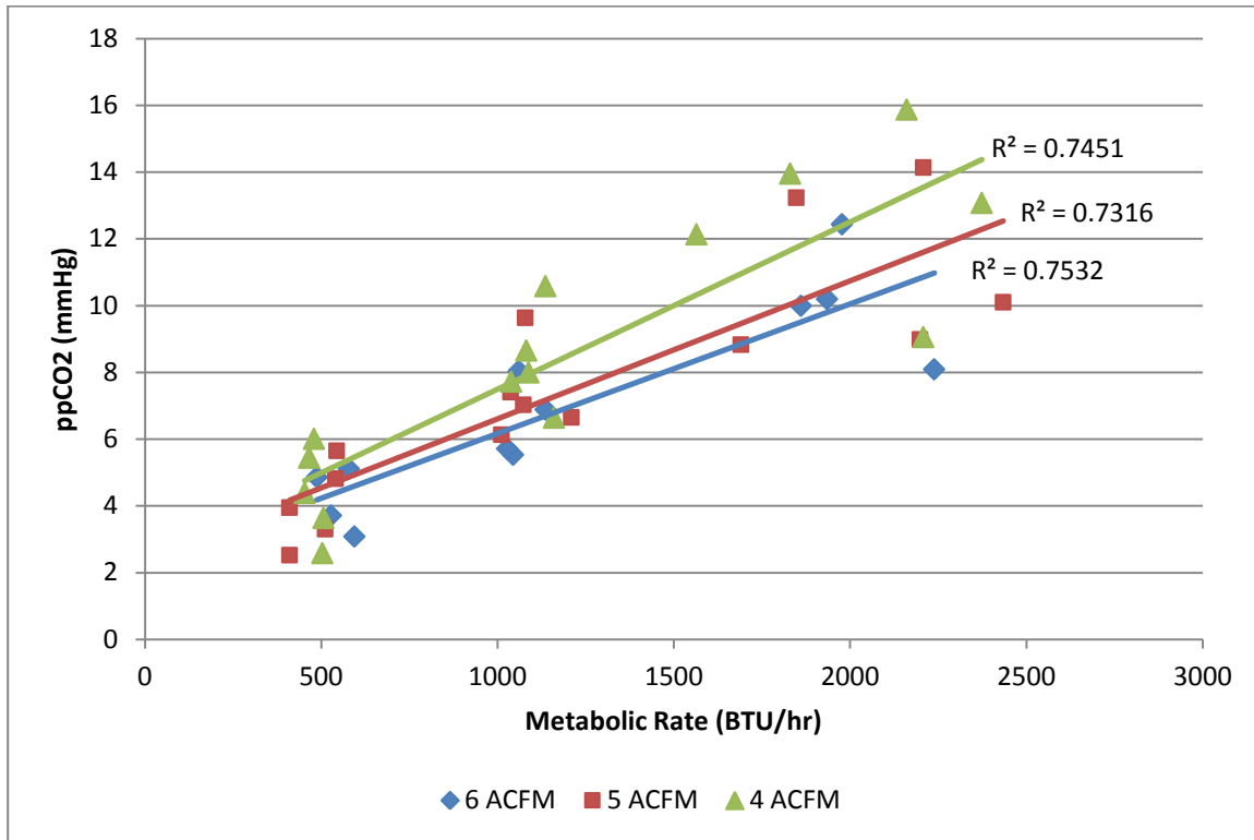
Figure 15. Inspired oronasal ppCO 2 as a function of metabolic rate for different EM-ACES suit flow rates.
