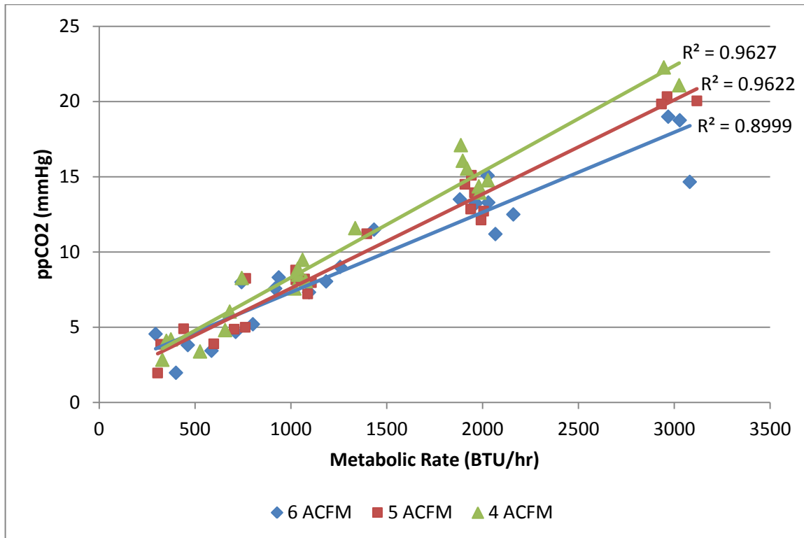
Figure 10. Inspired oronasal ppCO 2 as a function of metabolic rate for different REI suit flow rates.
