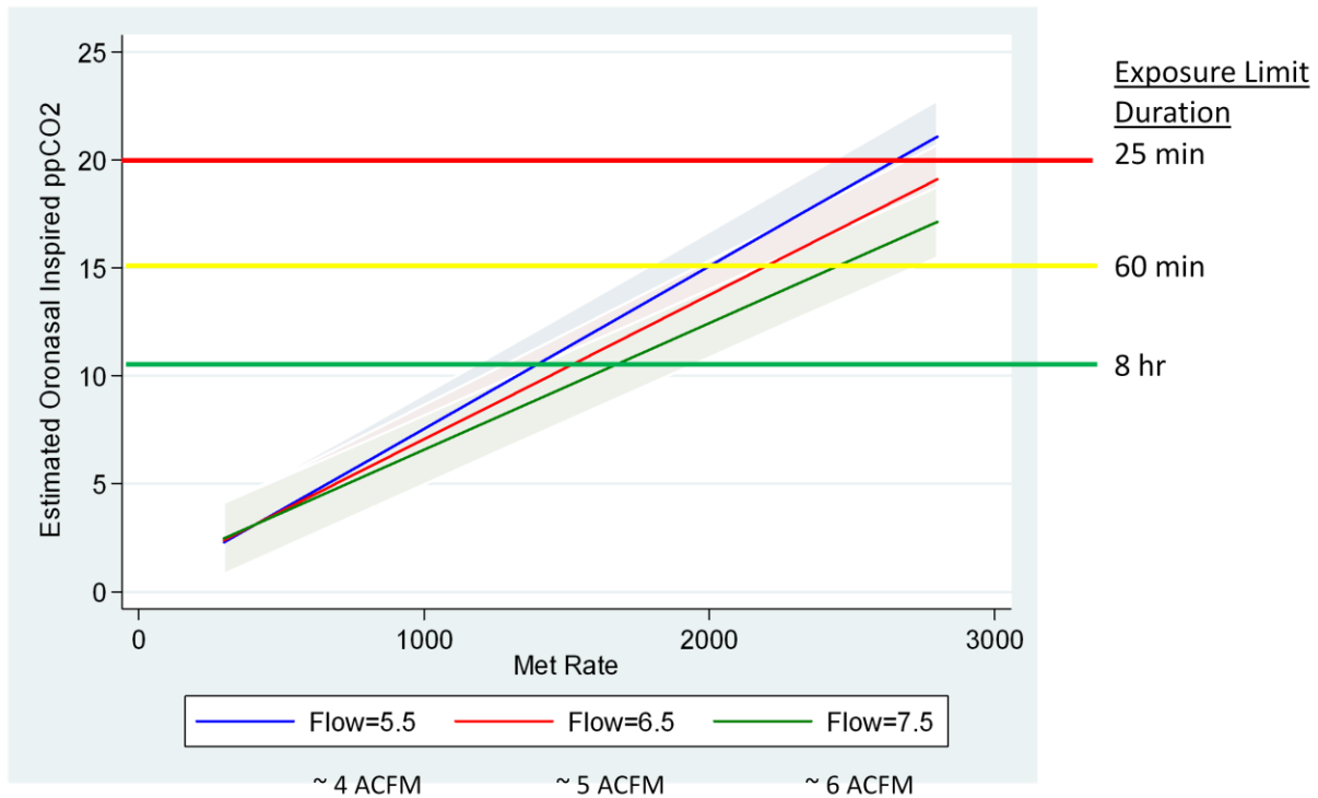
Figure 11. Statistical regression model showing the estimated inspired oronasal ppCO 2 at different metabolic and flow rates for the REI suit.
