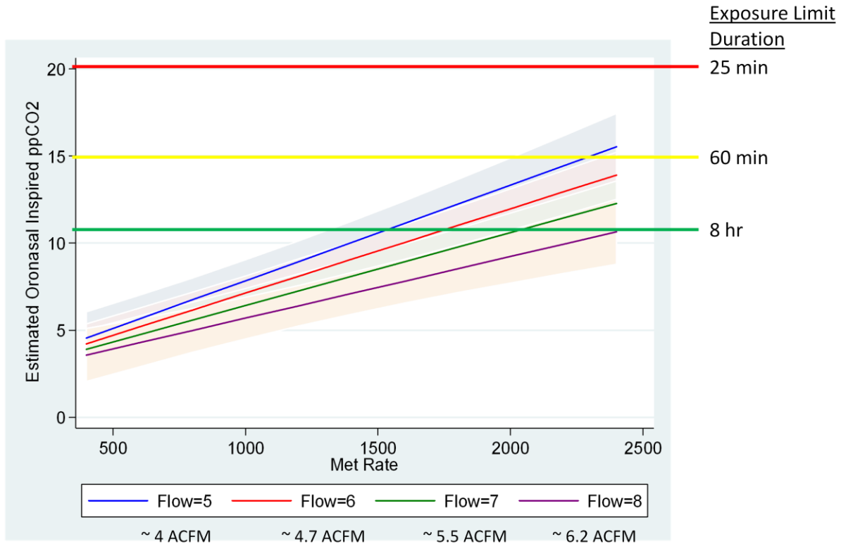
Figure 16. Statistical regression model showing the estimated inspired oronasal ppCO 2 at different metabolic and flow rates for the EM-ACES.
