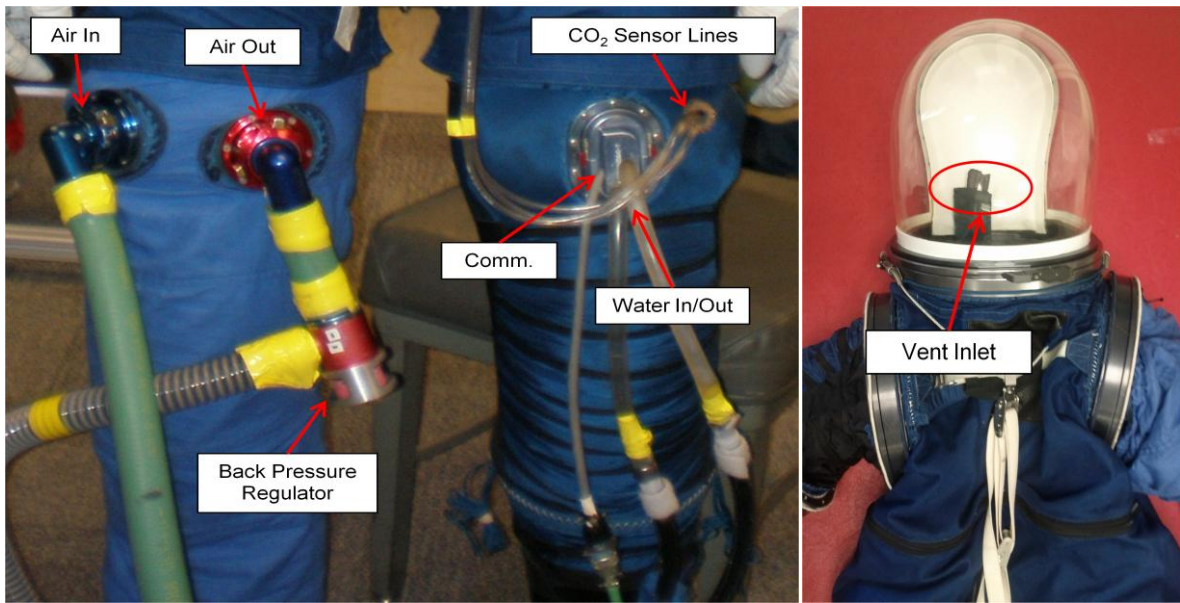
Figure 4. EM-ACES external interfaces.
