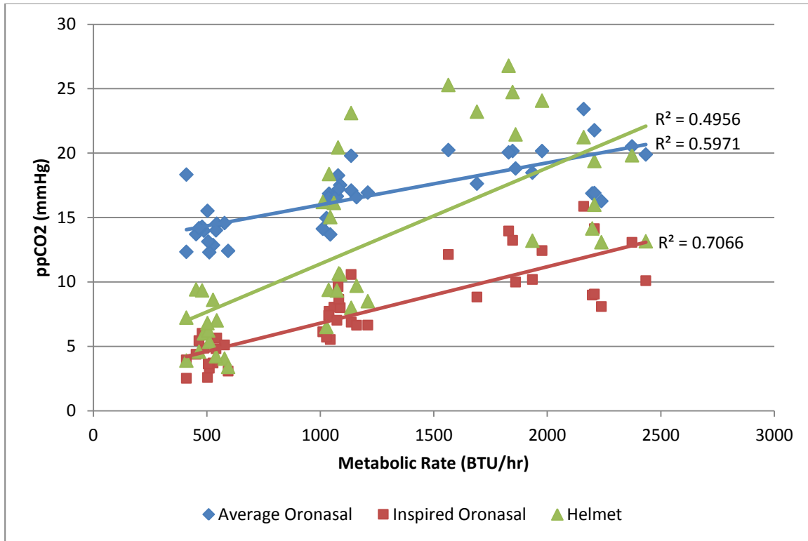
Figure 14. ppCO 2 variables as a function of metabolic rate during the EM-ACES CO 2 washout test.
