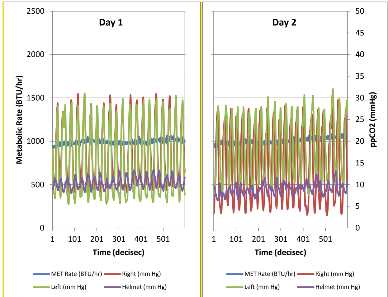
Figure 12. Example comparison of a test subject at the 1000 BTU/hr / 4 ACFM test points during the EM-ACES test. This example shows a bit of left/right variation between test days.
