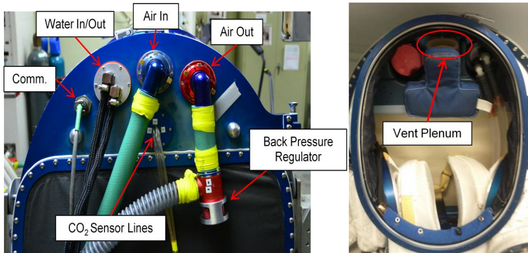
Figure 2. REI-suit external interfaces.
