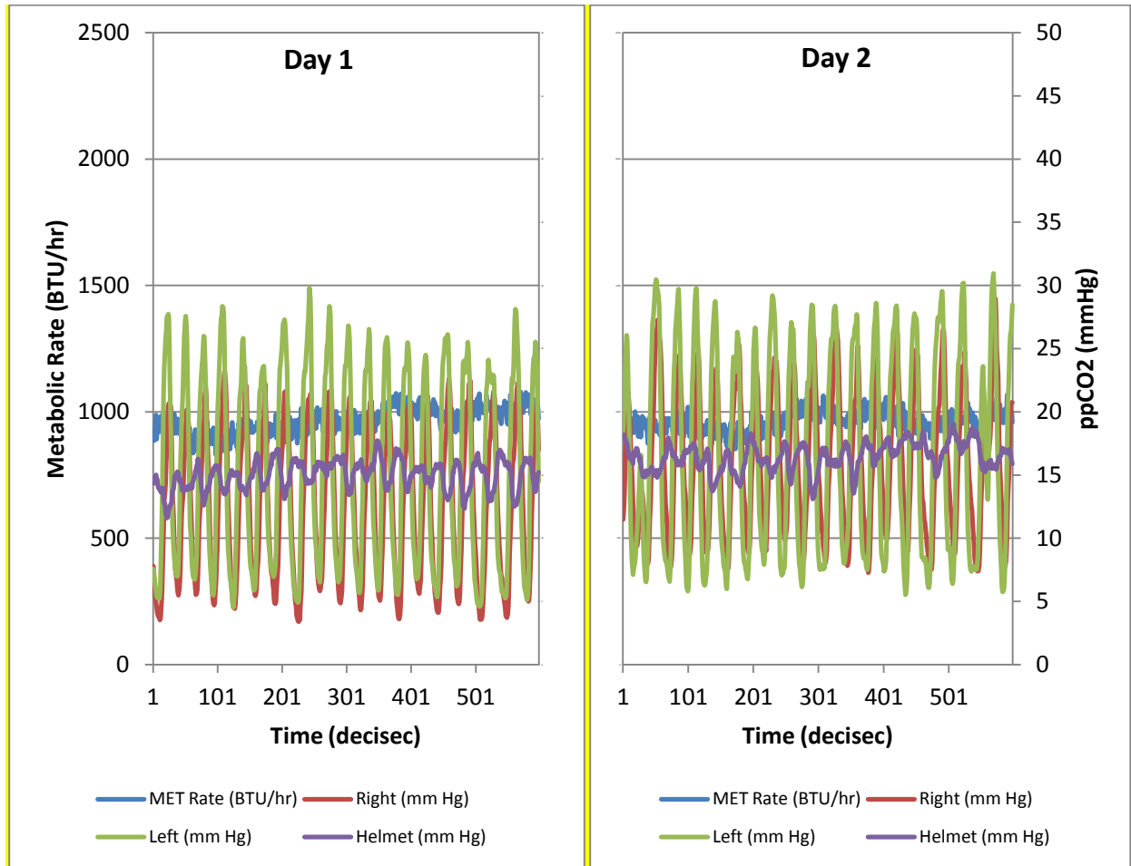
Figure 13. Example comparison of a test subject at the 1000 BTU/hr / 6 ACFM test points during the EM-ACES test. This example shows a slight upward shift from day 1 to day 2.
