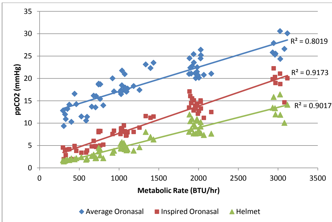
Figure 9. ppCO 2 variables as a function of metabolic rate in the REI-suit.
