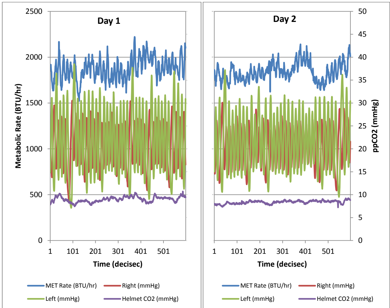
Figure 7. Example comparison of a test subject at the 2000 BTU/hr / 5 ACFM test points during the REI-suit test.
