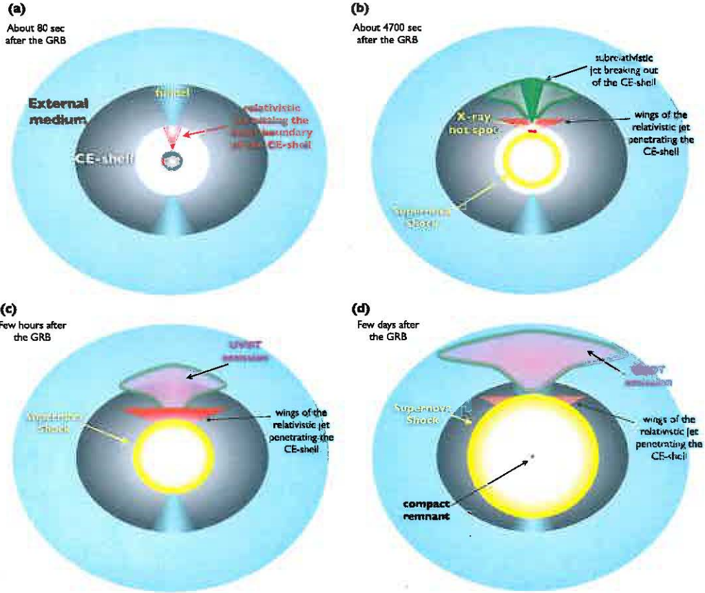
Figure 18: Cartoon of the different stages in our model of GRB 101225A. The different stages are explained in the text.
