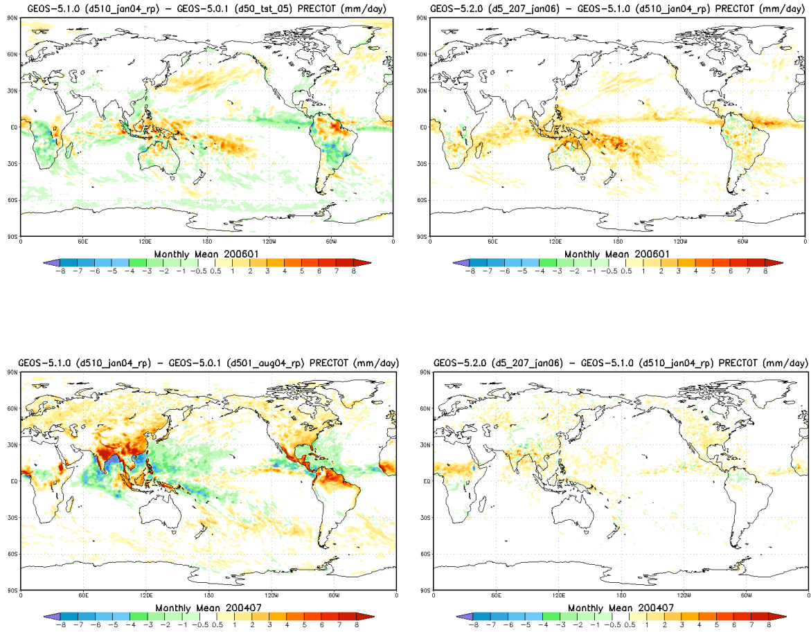
Figure 5.3.3: Mean difference in precipitation for January 2006 (upper panels) and July 2004 (lower panels) in mm/day. The left-hand panels show GEOS-5.1.0 minus GEOS-5.0.1. The right-hand panels show GEOS-5.2.0 minus GEOS-5.1.0.
