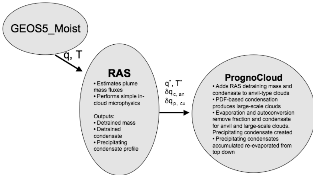
Figure 2.2.1: Schematic of Moist processes in GEOS-5.
