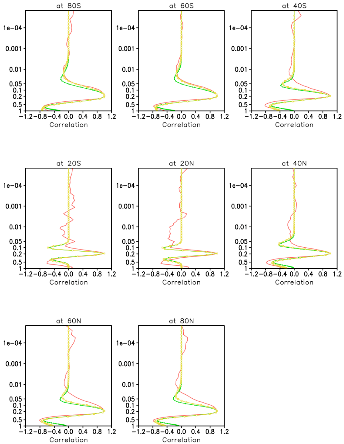
Figure 3.4.9: As in Figure 3.4.7, but for the correlation profiles at \sigma = 0.2 .
