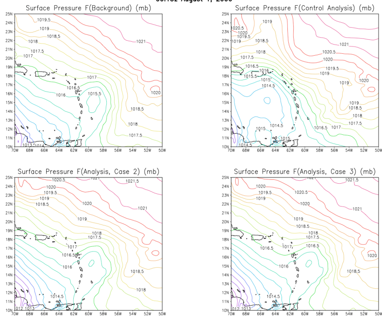
Figure 4.3.8: Surface pressure after 15 minutes of model integration, initialized from the background and analysis states (Control, Case 2, and Case 3).
