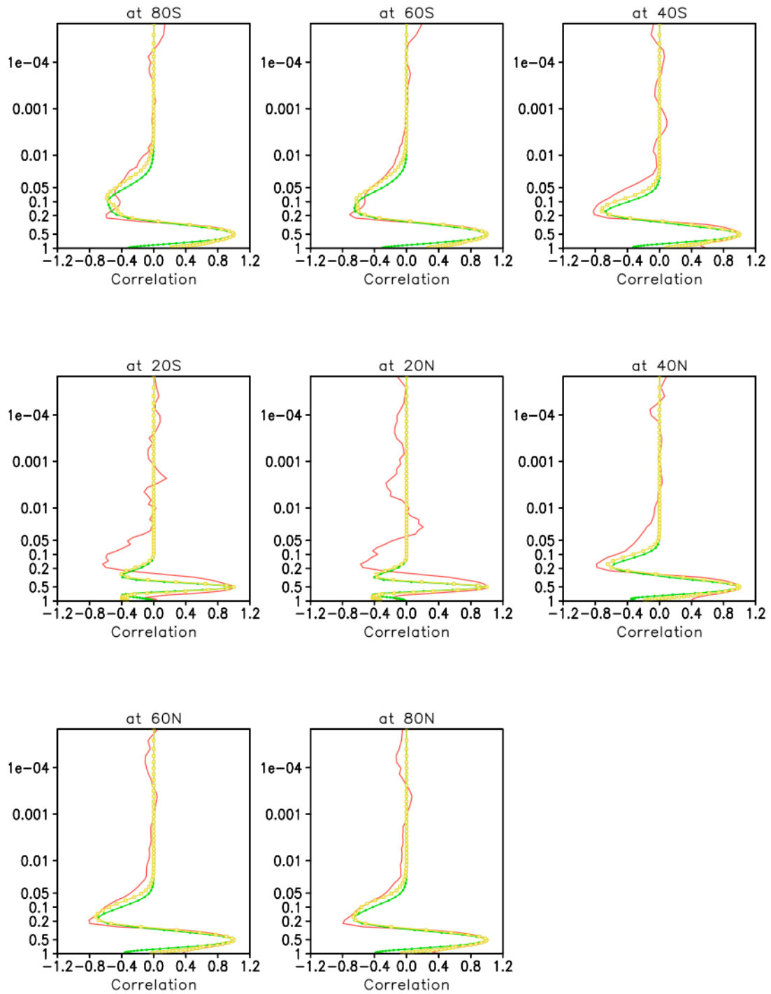
Figure 3.4.8: As in Figure 3.4.7, but for the correlation profiles at \sigma = 0.5 .
