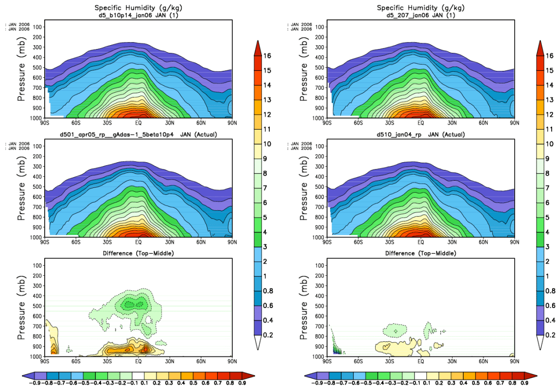
Figure 5.3.5: As in Figure 5.3.4, but zonal mean specific humidity (g/kg).
