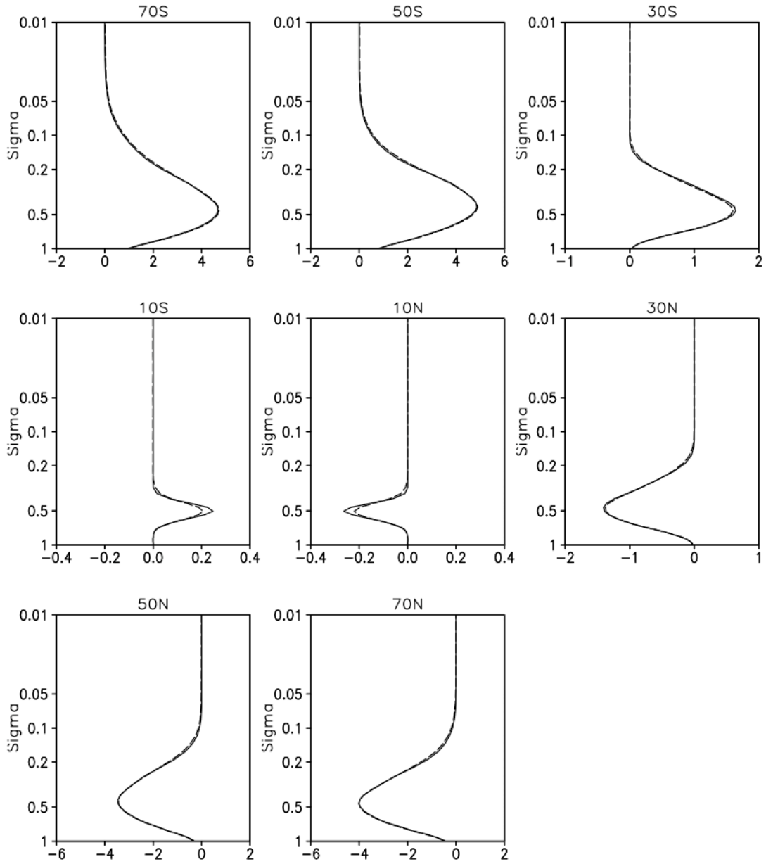
Figure 3.4.11a: As in Figure 3.4.6, but from the balanced projections estimated with the new approach used for GEOS.5.0.1.
