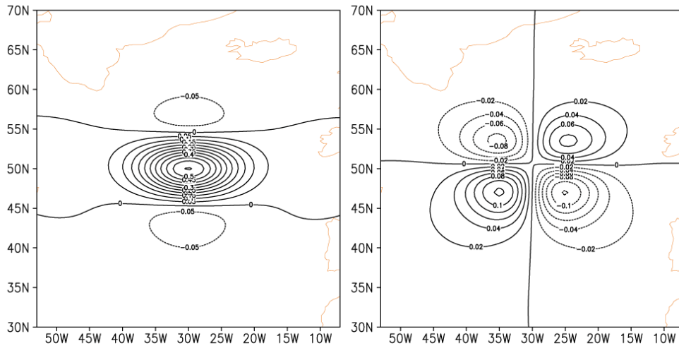
Figure 3.4.4: u (left) and v (right) increments ( x_a - x_b ), at sigma level 0.267, from a 1 m/s westerly wind observational residual ( y_o - h(x_b) ) at 50°N and 330°E at 250 hPa.
