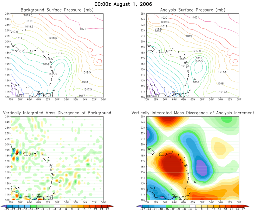
Figure 4.3.2: Surface pressure for the background and analysis states (upper panels). Also shown are the vertically integrated mass-divergence (arbitrary units) of the background (left-hand lower panel) and the (analysis-background) difference (right-hand lower panel).
