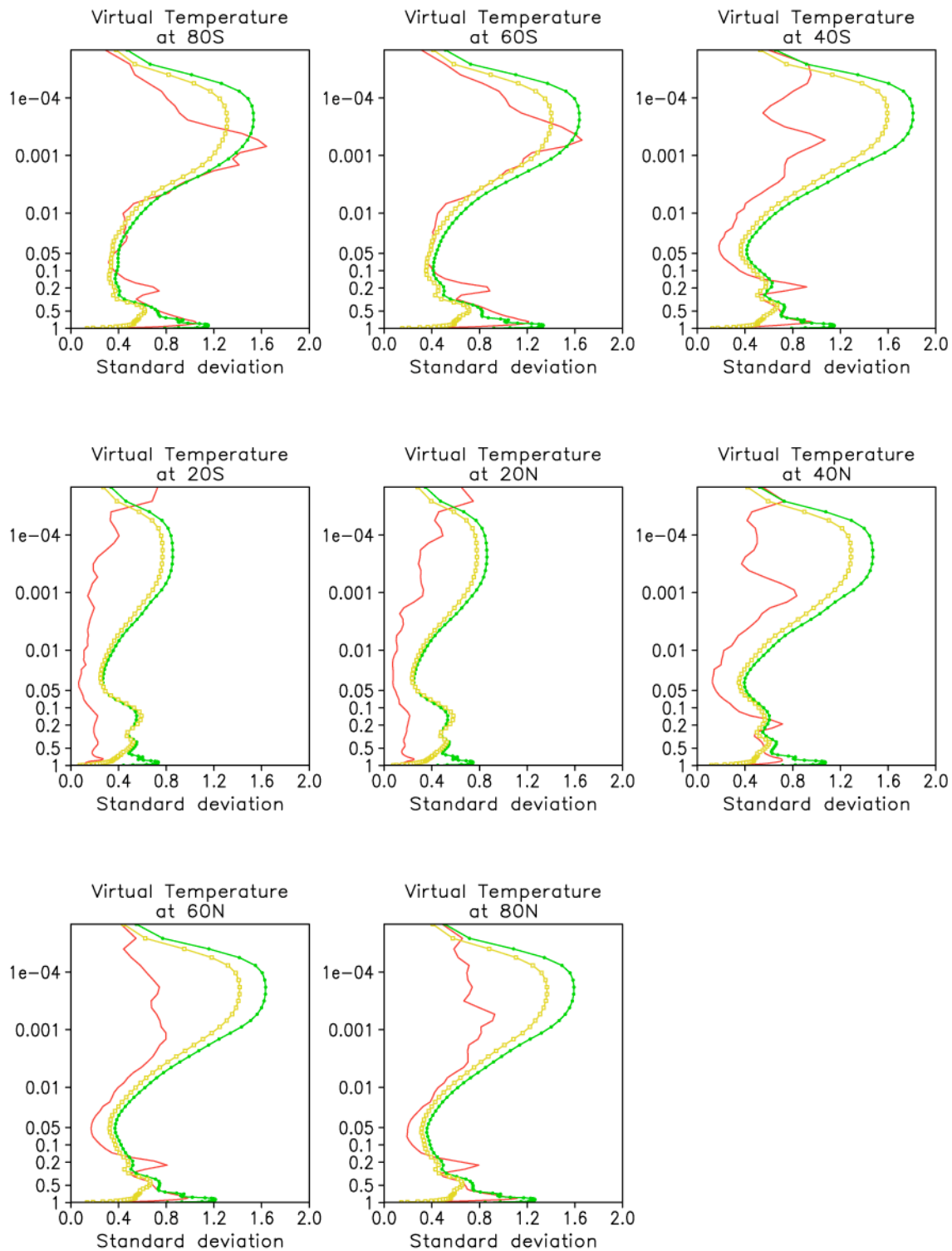
Figure 3.4.7: The standard deviation profiles of balanced temperature as a function of sigma at eight selected latitudes. The red curves are the estimates from the original GSI implementation, while the other curves are from the new approach. The green (yellow) curve shows the statistics used in GEOS-5.0.1 (GEOS-5.1.0).
