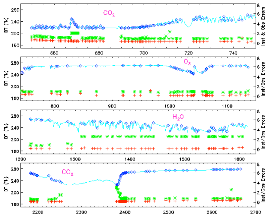
Figure 3.5.1: AIRS observed brightness temperatures for all 2378 channels are shown in light blue. The spectral location (blue diamond), instrument noise (red cross), and the assigned observation errors (green asterisk) in GSI for the 281-channel subset are also shown.
