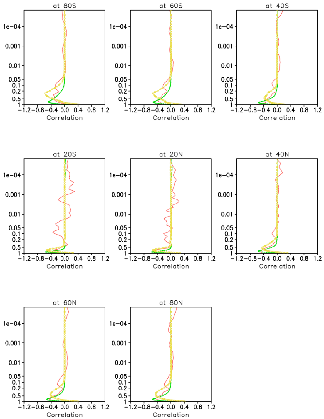
Figure 3.4.10: As in Figure 3.4.9, but for the cross-correlation profiles between the balanced temperature and balanced surface pressure.
