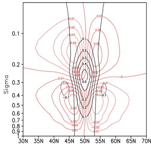
Figure 3.4.5: The vertical cross-section of u and T increments for the observation used for Figure 3.4.4.
