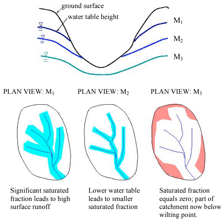
Figure 2.2.5: Separation of the catchment area into hydrological regimes.
