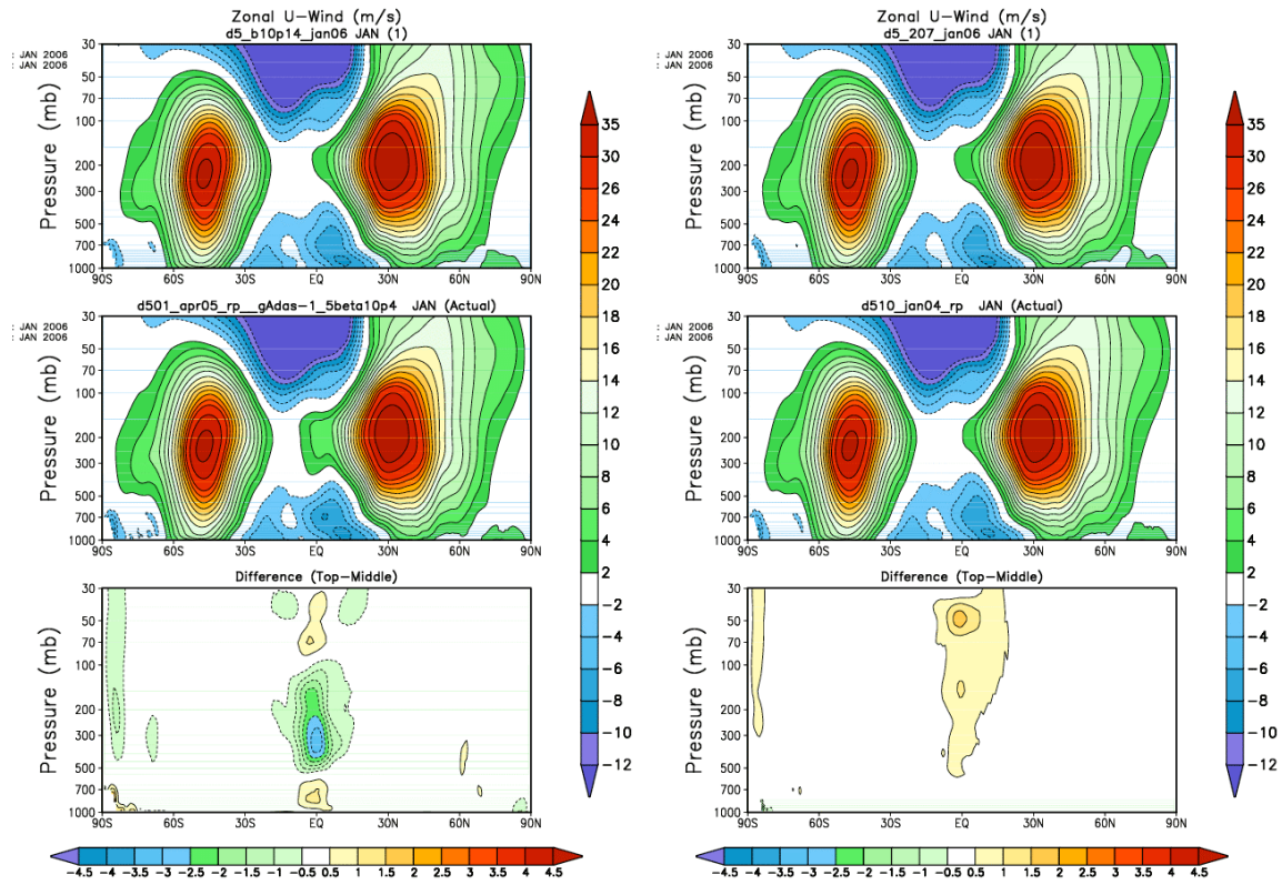
Figure 5.3.6: As in Figure 5.3.4, but zonal mean zonal wind ( \text{m s}^{-1} ).
