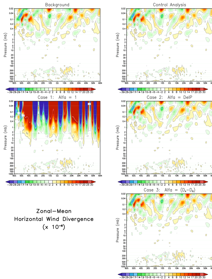
Figure 4.3.5: The zonal mean horizontal wind divergence (plotted on constant pressure surfaces) of the background state (from the model first guess) and the corresponding results from the analysis states.
