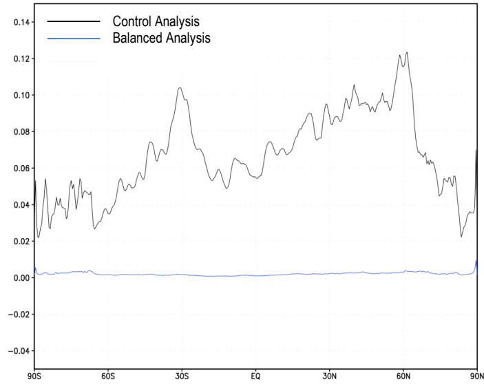
Figure 4.3.4: Zonal mean of the absolute value of the vertically integrated mass divergence analysis increment.
