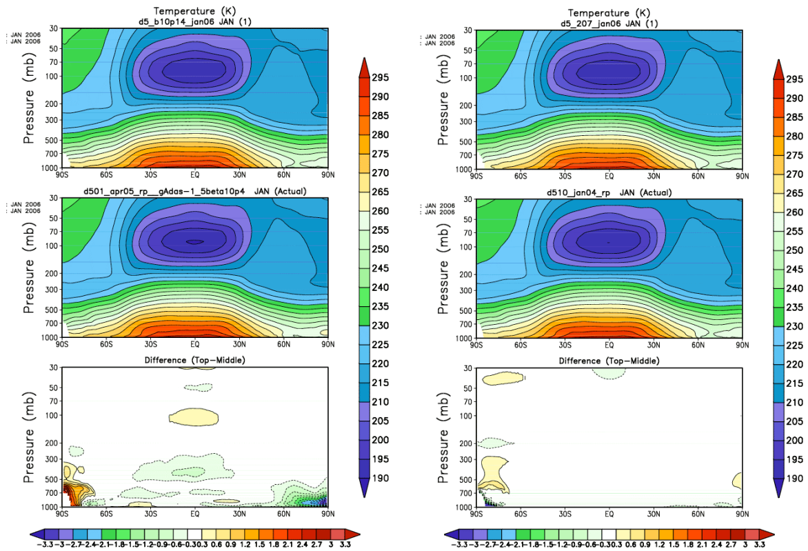
Figure 5.3.4: Zonal mean temperature (K) for January 2006. The left-hand figure shows GEOS-5.1.0 (upper panel), 5.0.1 (middle panel) and the difference (5.1.0 minus 5.0.1, lower panel). The right-hand figure shows GEOS-5.2.0 (upper panel), 5.1.0 (middle panel) and the difference (5.2.0 minus 5.1.0, lower panel).
