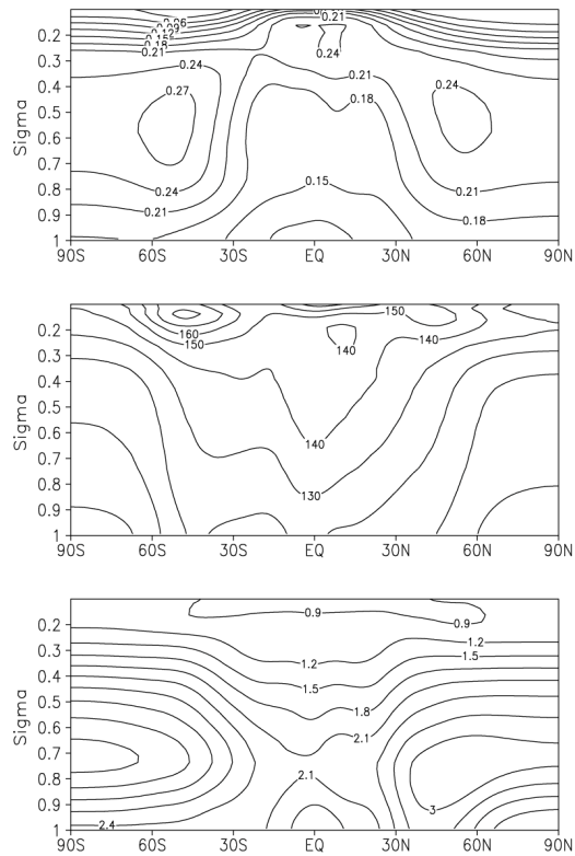
Figure 3.4.3: Example of estimated background error statistics for pseudo-relative humidity. Top: error standard deviation as a function of latitude and sigma level; middle: horizontal scales of covariance (in km); bottom: vertical scale factors for covariance.
