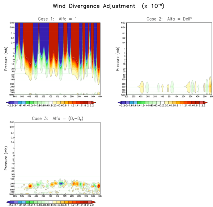
Figure 4.3.7: The zonal mean of the adjustment made to the control analysis of horizontal divergence.
