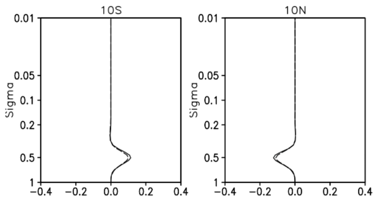
Figure 3.4.11a: As in Figure 3.4.6, but from the balanced projections estimated with the new approach used for GEOS.5.0.1.
