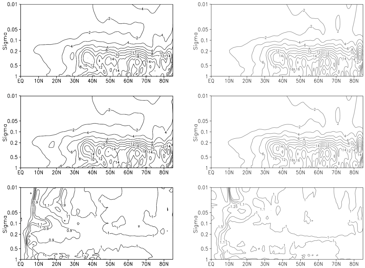
Figure 3.4.12: Zonal averages of |L_\Phi| \equiv |\nabla^2 \delta\Phi| (top), |R_\Psi| \equiv |\nabla \cdot (f \nabla \delta\psi)| (middle). L_\Phi and R_\Psi are calculated based on the analysis increments which only includes the wind-mass balance projections with the new approach. All the values in the top and middle have been multiplied by 10^{10} . The bottom panel displays the ratio of top field to the middle, the contours of 0.5, 0.75, 0.9, 1.0, 1.1, 1.25, 1.5, 2.0, 4.0, 6.0 are plotted. Left-hand panels are for GEOS-5.0.1; right-hand panels are for GEOS-5.1.0.
