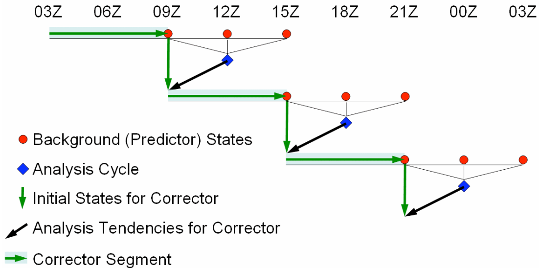
Figure 4.2.1: A schematic of the IAU implementation.
