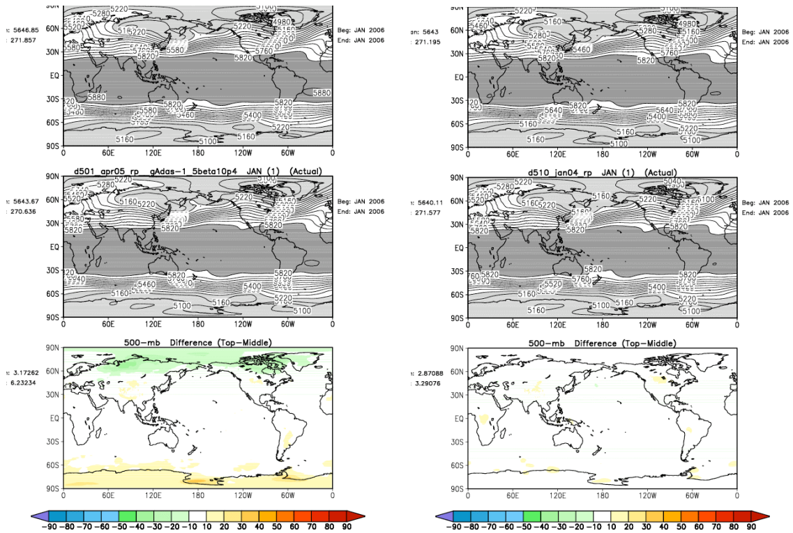
Figure 5.3.2: As in Figure 5.3.1, but for 500-hPa height. The mean difference is between 5.1.0 and 5.0.1 is 3.2 hPa, and the standard deviation of the difference is 6.2 hPa. The mean difference is between 5.2.0 and 5.1.0 is 2.9 hPa, and the standard deviation of the difference is 3.3 hPa.
