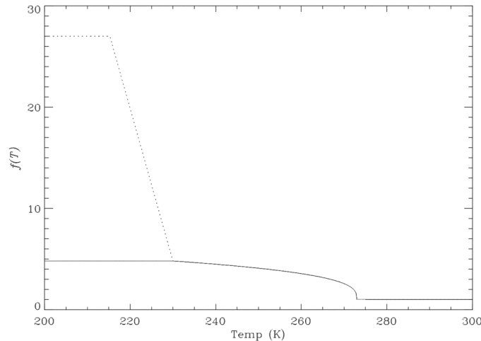
Figure 2.2.3: “Sundqvist-factor” controlling low-temperature autoconversion.
