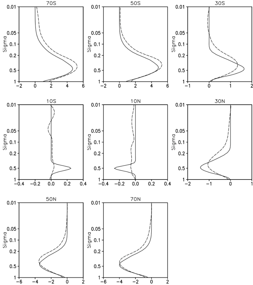
Figure 3.4.6: The profiles of \langle \delta\psi, \nabla^2 \delta\Phi \rangle (dashed line) and \langle \delta\psi, \nabla \cdot (f \nabla \delta\psi) \rangle (solid line) at eight selected latitudes with \delta\psi being at \sigma = 0.5 . These profiles are calculated from the balance projection coefficients estimated according to the original GSI implementation, and values have been multiplied by 10^3 .
