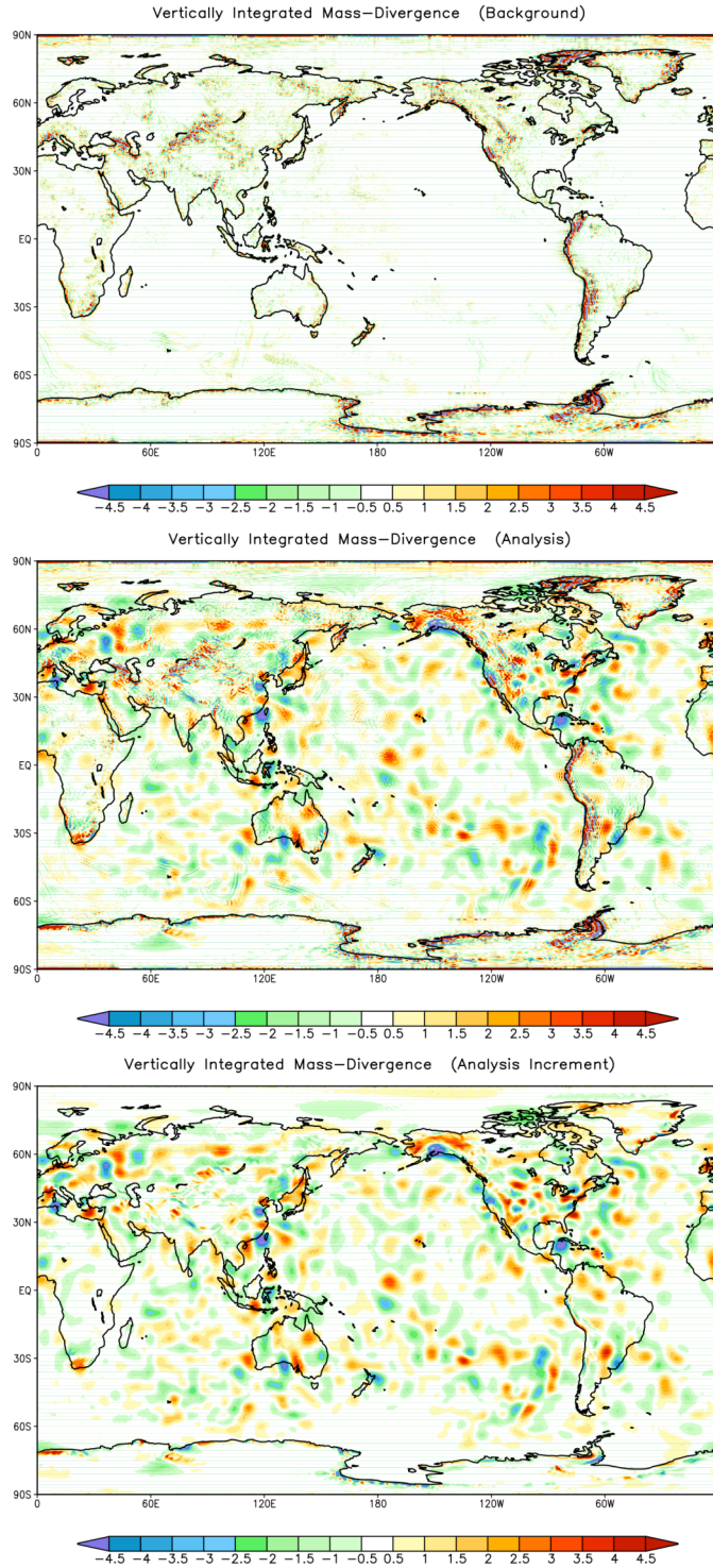
Figure 4.3.1: The vertically integrated mass-divergence (in arbitrary units) on 1 August, 2006 for the background (top), the analysis state (middle) and from the difference, or analysis increment (bottom).
