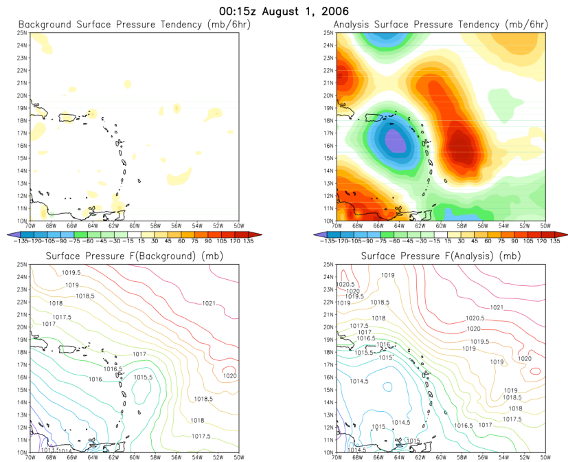
Figure 4.3.3: Surface pressure tendency of the background (left-hand upper panel) and analysis states (right-hand upper panel), and the resulting surface pressure after 15 minutes of model integration from the background without analysis (left-hand lower panel) and from the analysis (right-hand lower panel).
