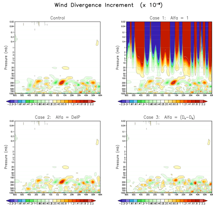
Figure 4.3.6: The zonal mean of the analysis increment of divergence.
