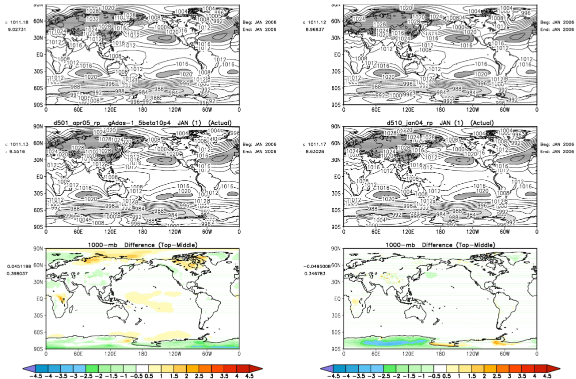
Figure 5.3.1: Mean sea-level pressure for January 2006. The left-hand figure shows GEOS-5.1.0 (upper panel), 5.0.1 (middle panel) and the difference (5.1.0 minus 5.0.1). The mean difference is 0.05 hPa, the standard deviation of the difference is 0.40 hPa. The right-hand figure shows GEOS-5.2.0 (upper panel), 5.1.0 (middle panel) and the difference (5.2.0 minus 5.1.0). The mean difference is 0.05 hPa, the standard deviation of the difference is 0.35 hPa.
