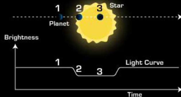
Transit Method
