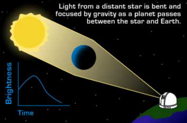
Gravitational Microlensing
