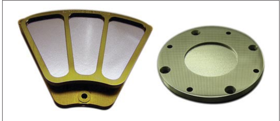
SUVI (Solar Ultraviolet Imager) Entrance Filter Prototype —150 nm Al on 70 lpi polyimide mesh and an ASTRO-H DMS filter prototype — 80 nm Al on 100 nm polyimide with 70 lpi polyimide mesh.
