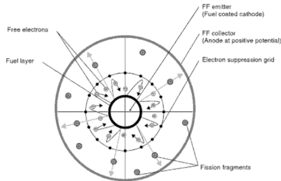
Figure 47.4 "Triode" FEC design.
