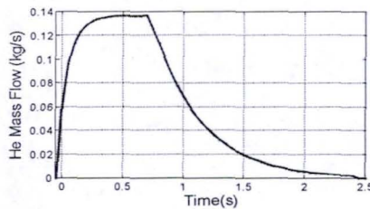
Fig. 2-6: The form of the He mass flow pulses.
