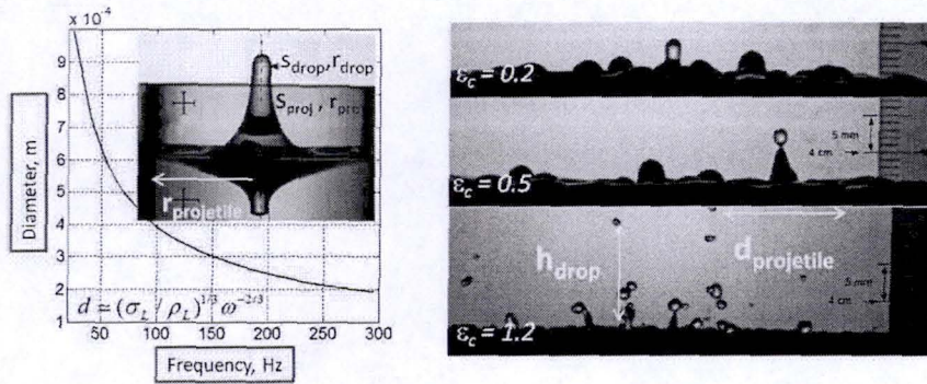
Fig.6-5. Typical diameter of ejected droplets depending on thrust oscillation frequency (left) and generation of droplets under action of supercritical vibration acceleration \varepsilon_d > 0 [13].
