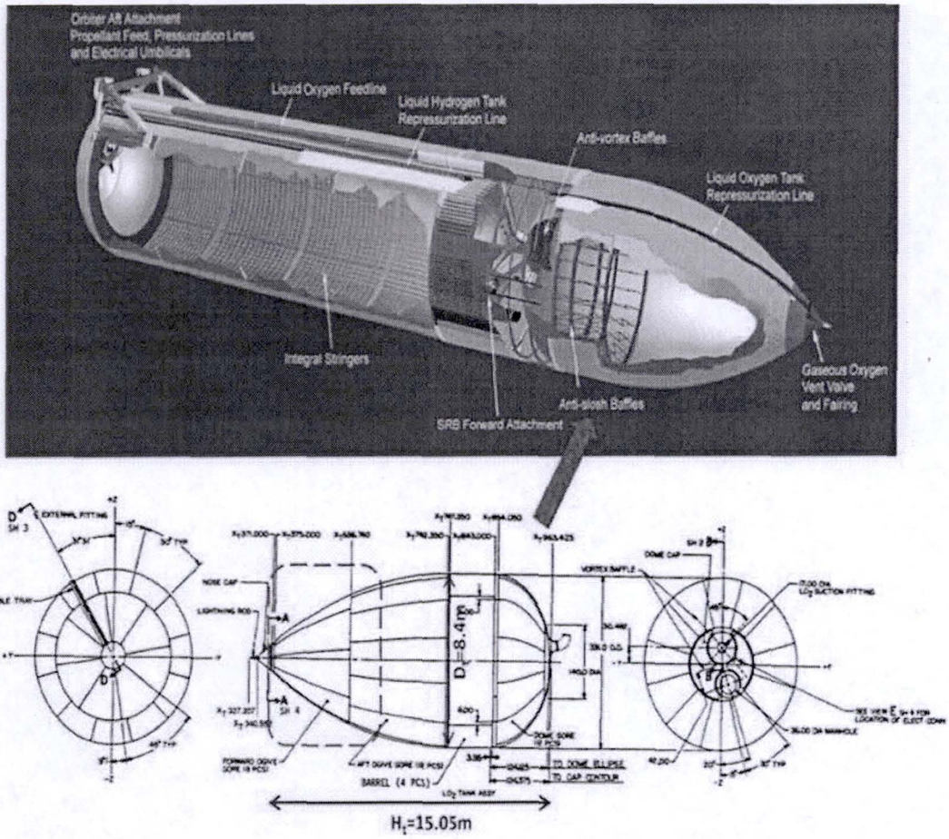
Fig.1. Design of the Shuttle tanks: the shape and parameters of the LOx tank
