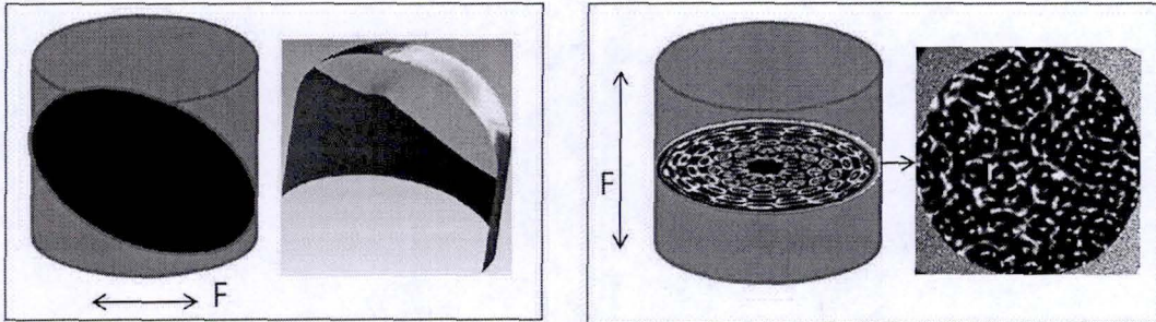
Fig.6-1 Two main types of sloshing: (i) Longitudinal sloshing waves excited by lateral forces (left); (ii) Axial sloshing (capillary waves) excited parametrically by axial vibrations (right)
