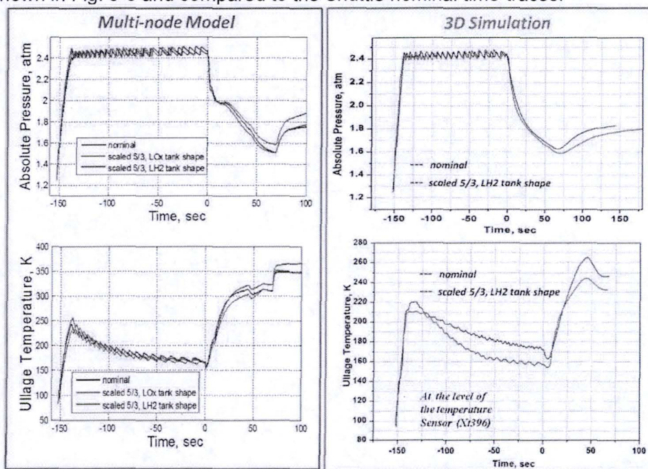
Fig.5-3 Predicted time traces of ullage pressure and temperature for different shapes of the SLS LOx tanks. Results of MMN and 3D simulations.
