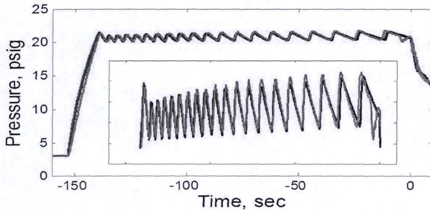
Fig.2-7: Ullage pressure during the pre-pressurization: STS115DB telemetry (red) and MNM simulation (blue). Results of the fitting with \beta_u=0.05 , \tau_{\text{front}} = 0.09 \text{ sec} , \tau_{\text{tail}} = 0.5 \text{ sec} , and \tau_{\text{pulse}} = 0.7 \text{ sec} .
