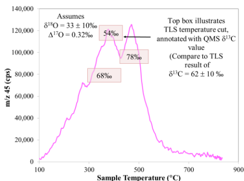
Figure 2. CO 2 released from Rocknest 4 soil sample. QMS results for δ 13 C are shown in pink text boxes. See text for details.
