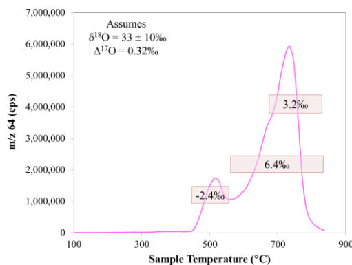
Figure 3. SO 2 released from Rocknest 1 soil sample. QMS results for δ 34 S are shown in pink text boxes. See text for details.
