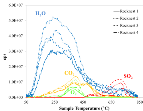
Figure 1. Major volatiles released from Rocknest soil.
