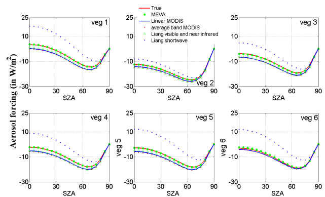
Fig. 13. Aerosol forcing when SZA varies from 0 to 90 degrees for vegetation types shown in Fig. 9. Curves in different symbols are associated with different approaches to estimate vegetation reflectance spectrum used in the aerosol forcing calculation. Other parameters used in the calculations include AOD (at 0.55 μm) of 0.32 and SSA (at 0.55 μm) of 0.89.
