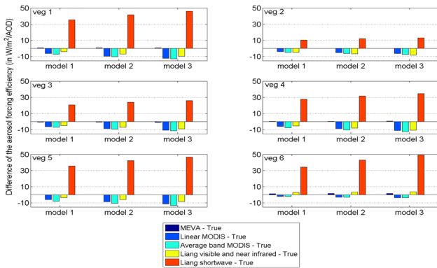
Fig. 11. Difference of the aerosol forcing efficiency (in W m^{-2} AOD^{-1} ) associated with different approaches to estimate reflectance spectra for vegetation types shown in Fig. 9. In each subplot, three groups indicate the results caused by using three different aerosol models shown in Fig. 10: SSA (at 0.55 μm) = 0.95 (noted as “model 1”), 0.89 (noted as “model 2”), and 0.83 (noted as “model 3”). Other parameters used in the calculations include AOD (at 0.55 μm) = 0.32 and SZA = 30 degrees.
