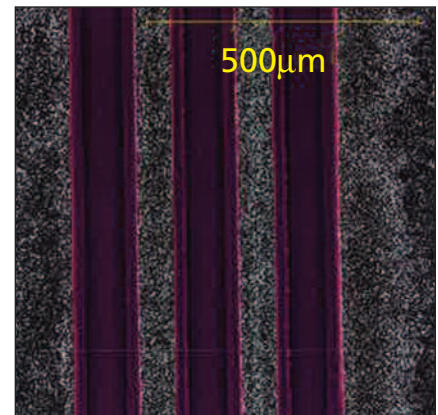
Microchannels in a 150- \mu\text{m} thick GGG disk fabricated by ultra-short pulse laser micromachining.
