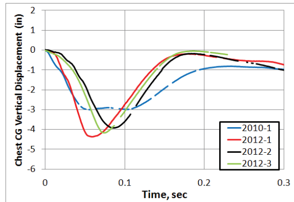
Figure 14 - Chest CG vertical displacement for four different input pulses
