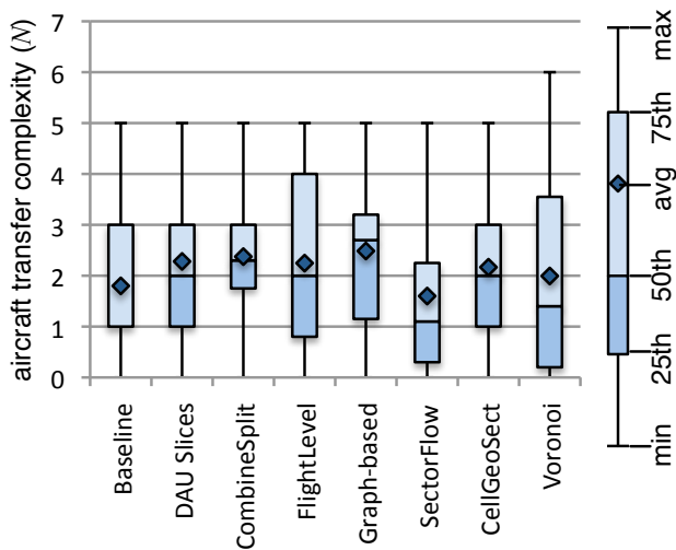
Figure 11: N averages and quartiles across the first reconfiguration ( c_1 to c_2 ) for each airspace design method.
