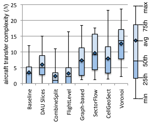
Figure 12: N averages and quartiles across the second reconfiguration ( c_2 to c_3 ) for each airspace design method.
