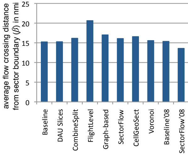
Figure 7: \beta values for each airspace design method.
