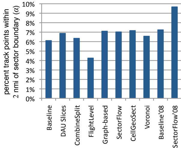
Figure 6: Average \alpha values for each airspace design method.
