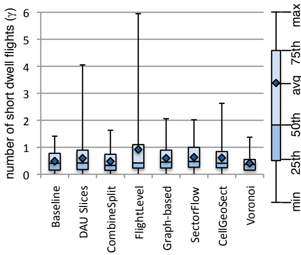
Figure 8: \gamma averages and quartiles for each airspace design method.
