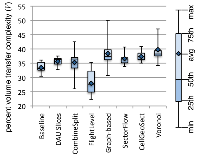
Figure 9: V averages and quartiles for all mapped sectors across the first reconfiguration ( c_1 to c_2 ) for each airspace design method.
