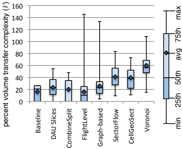
Figure 10: V averages and quartiles for all mapped sectors across the second reconfiguration ( c_2 to c_3 ) for each airspace design method.
