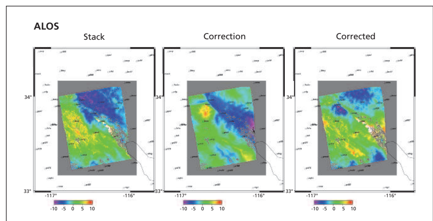
Advanced Land Observing Satellite (ALOS) Data. At left, the original stack of 33 interferograms. Center: The stacked correction maps, showing typical distribution of moisture in the Coachella Valley, CA. At right, the corrected stacked image.
