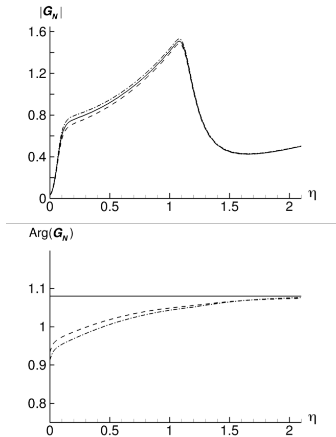
Figure 16. The effect of wall impedance on the magnitude (top) and phase (bottom) of the GF – (rigid: solid line); (1 + 0.50i) : dashed line; and (1 - 0.50i) : dash-dot at (\phi = \pi/2, \theta = \pi/4, St_o = 0.30, U_j/c_\infty = 0.90, T_R = 1.0) .
