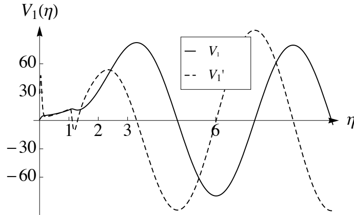
Figure 7. Solution V_1(\eta) (solid line) and its derivative (dashed line) subject to the mean velocity and temperature profiles of Figs 5 and 6 at ( \phi = \pi/2, \theta = \pi/4, St_o = 0.30, U_j/c_\infty = 0.90, T_R = 3.0 ).
