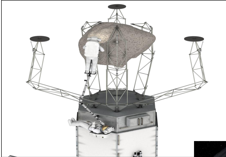
EVA crew member accessing asteroid on Alternate Concept capture mechanism.
