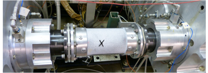
Figure 4.—Composite tube in machine with the most severe damage “X” notch.
