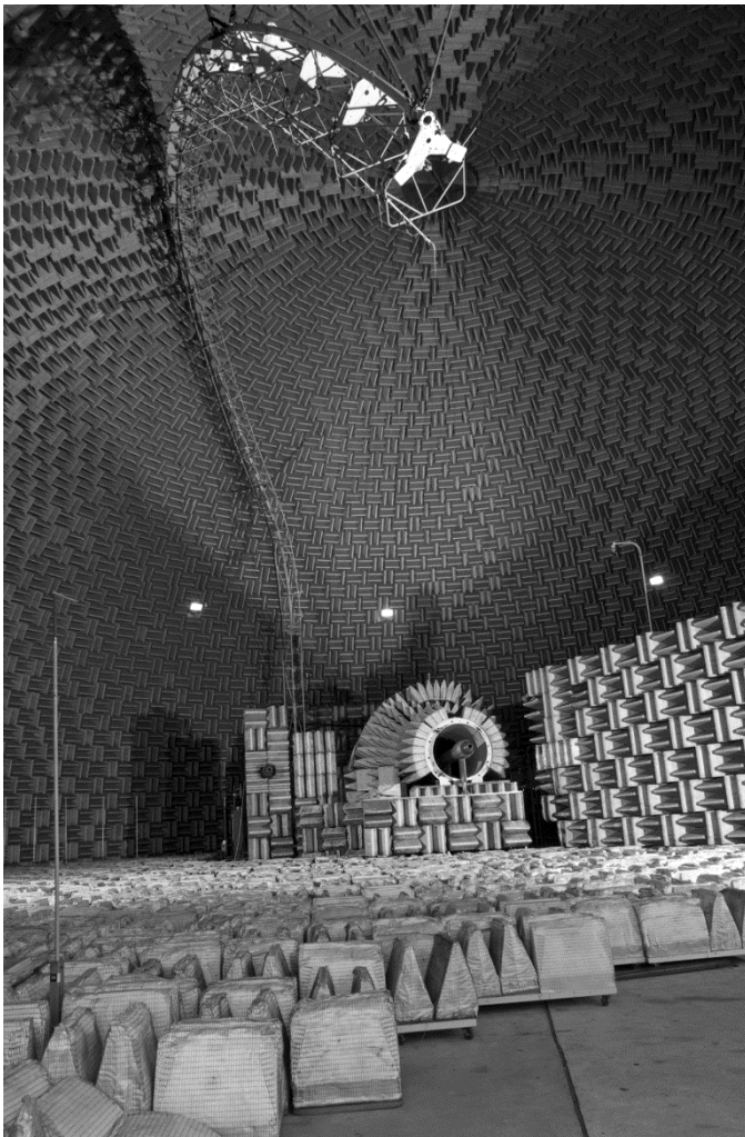
Figure 13.—Nozzle Acoustic Test Rig (NATR).
