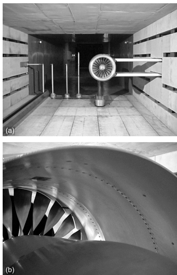
Figure 38.—Source diagnostics test (SDT). (a) External nacelle support struts. (b) Fan with no stators; view looking toward inlet from aft bypass duct.
