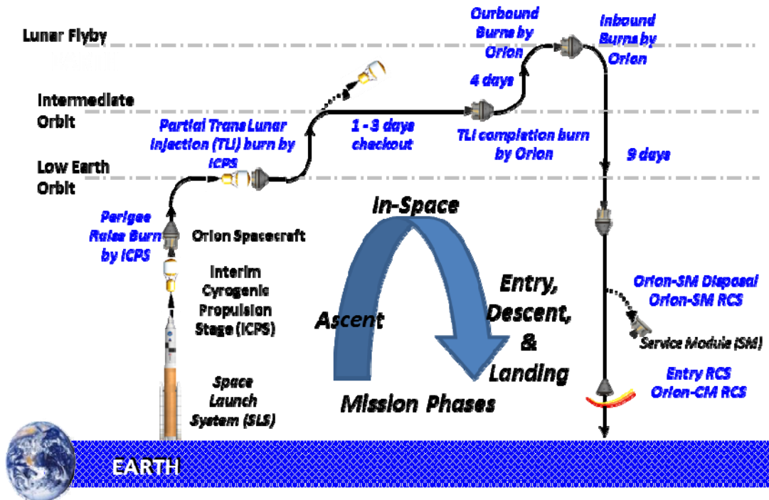
Figure 1: Hybrid Crewed Lunar Flyby DRM Chart
