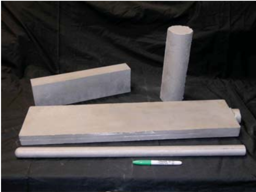
Figure 5 - Cast 60NiTi plate and rod ingots. Forward most cast rod used to produce indentation specimens tested in the present study.
