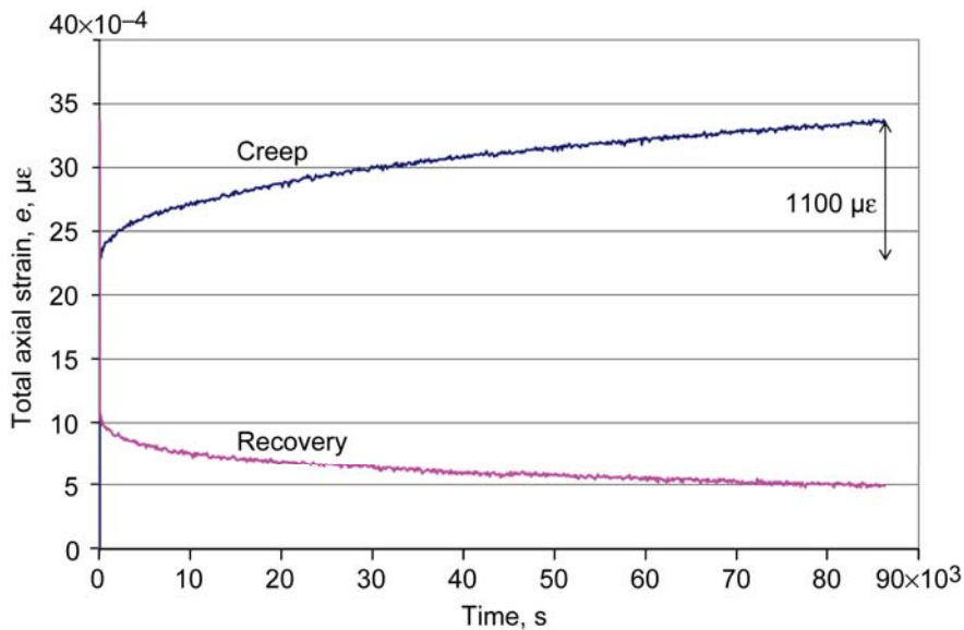
Figure 29.—Viscoelastic creep (stress \bar{\sigma} = 206 MPa) and recovery ( \bar{\sigma} = 0 MPa) of Ti-6Al-4V in irreversible regime at 427 °C (creep rate \dot{e}_c = 6.0 \times 10^{-9} s ^{-1} and recovery rate = -2.3 \times 10^{-9} s ^{-1} ).
