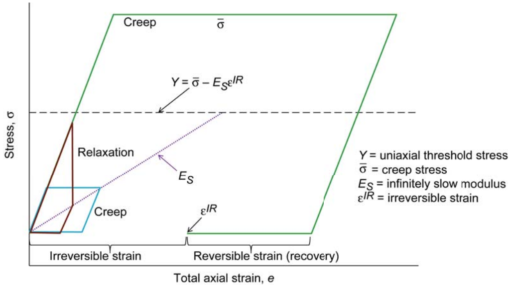
Figure 5.—Schematic depicting required testing for key viscoelastic parameters of Ti-6Al-4V.
