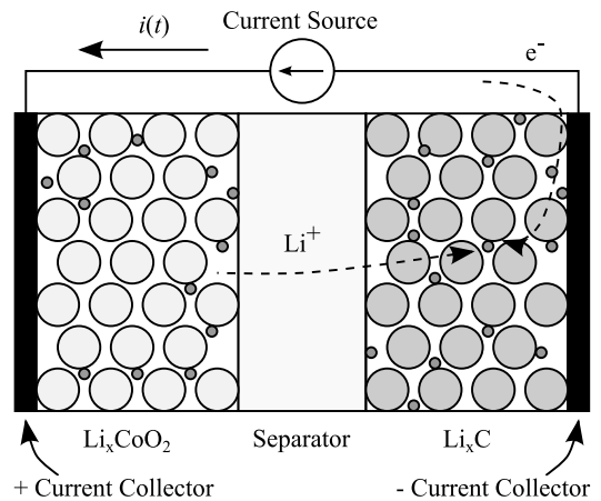
Figure 2. Li-ion battery during charge.
