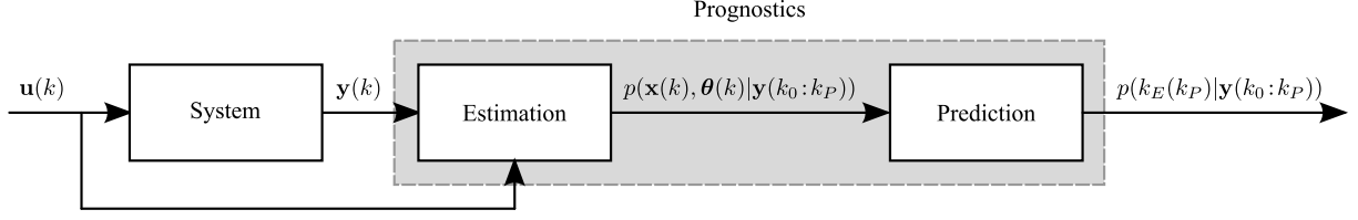
Figure 3. Prognostics architecture.
