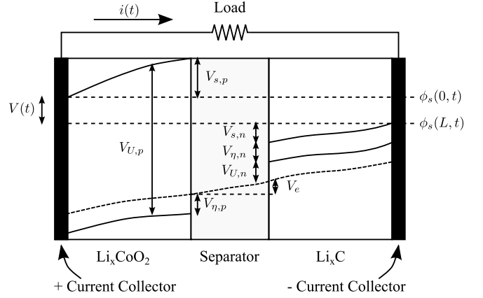
Figure 4. Battery voltages.
