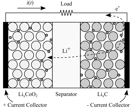
Figure 1. Li-ion battery during discharge.
