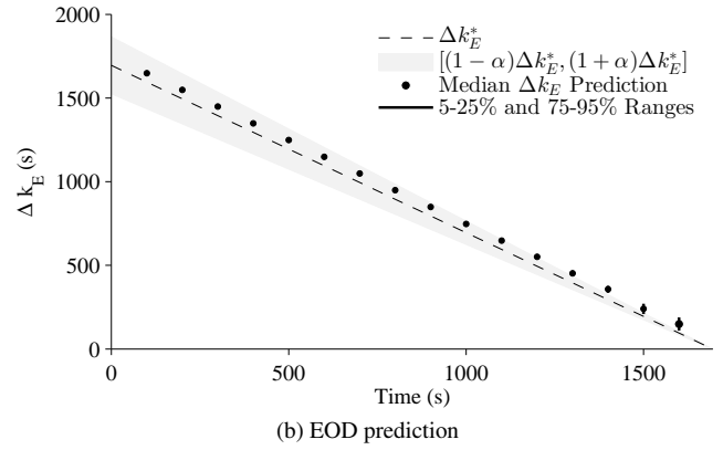
Figure 15. Prognostics results for variable loading discharge.
