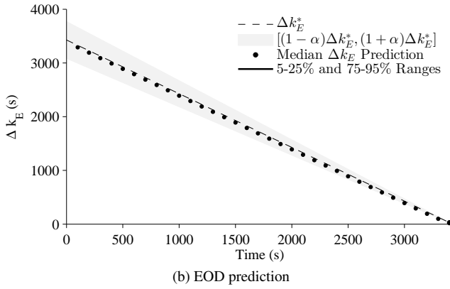
Figure 14. Prognostics results for 3 A discharge.
