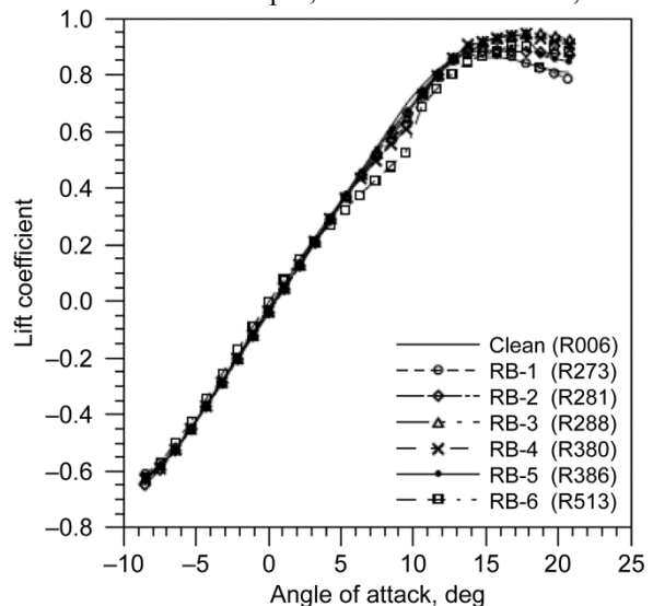
Fig. 20 Effect of simulated spanwise-ridge ice shapes located at 15% chord on GLC-305 swept wing, Re = 1.8 \times 10^6 , after Papadakis et al. 27
