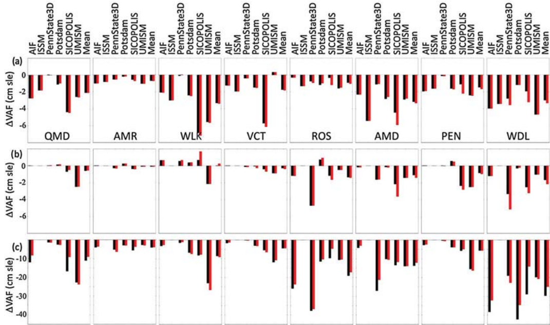
Figure 5. Comparison of the change in volume above flotation (experiment minus control) resulting from the suite of combination experiments to the sum of individual forcings for eight regions of the Antarctic ice sheet after 100 simulated years. (a) \Delta VAF_{C1S1} (black) versus \Delta VAF_{C1} + \Delta VAF_{S1} (red). (b) \Delta VAF_{C1M1} (black) versus \Delta VAF_{C1} + \Delta VAF_{M1} (red). (c) \Delta VAF_{C1S1M2} (black) versus \Delta VAF_{C1} + \Delta VAF_{S1} + \Delta VAF_{M2} (red).
