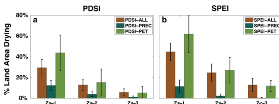
Fig. 13 Percent land area (excluding Antarctica) with annual average 2080–2099 PDSI (a) and SPEI (b) exceeding 1, 2, or 3 standard deviations. Bars represent the multi-model mean, and the error bars
