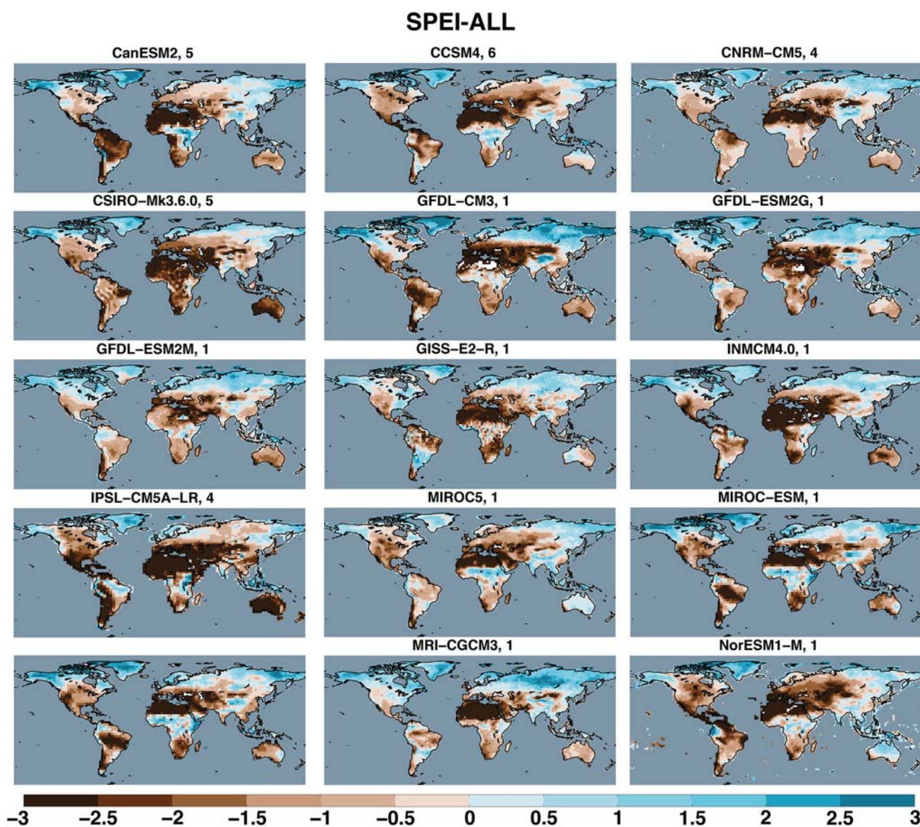
Fig. 6 Same as Fig. 5, but for SPEI-ALL
