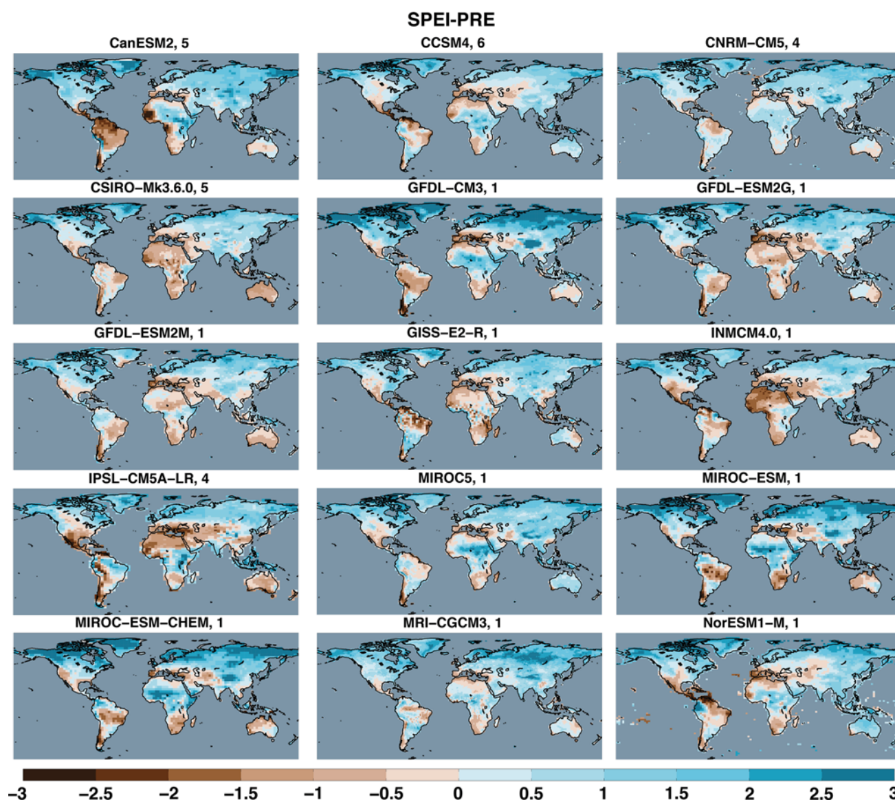
Fig. 8 Same as Fig. 7, but for SPEI-PRE
