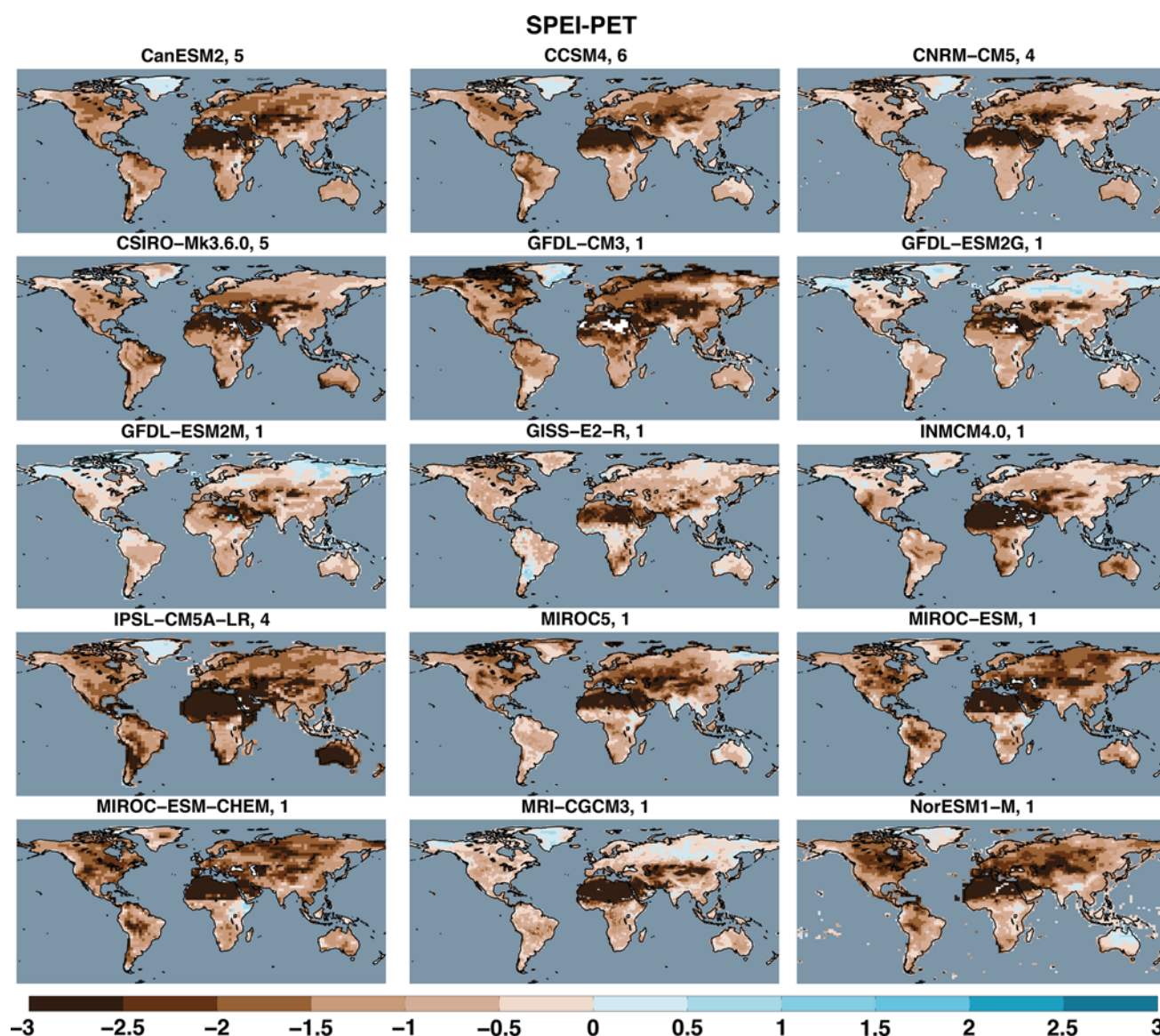
Fig. 10 Same as Fig. 9, but for SPEI-PET
