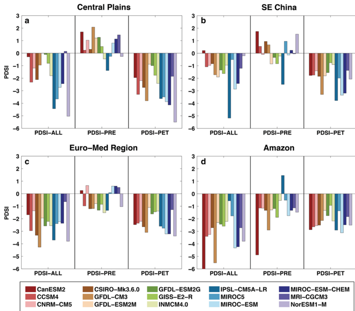
Fig. 15 Regionally averaged PDSI for each model, over a the Central Plains of North America (105° – 90°W, 32° – 50°N), b southeast China (102° – 123°E, 22° – 30°N), c the European-Mediterranean
