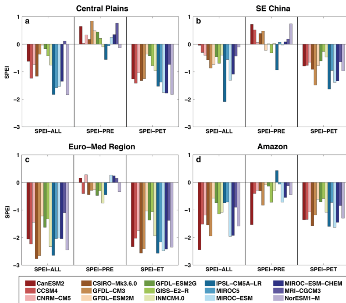
Fig. 16 Same as Fig. 15, but for SPEI
