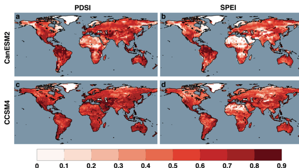
Fig. 1 Pearson's correlation coefficients calculated between PDSI (a,c) and SPEI (b,d) and annual average model soil moisture from the approximate top 30 cm of the soil column: CanESM2 (a,b) and CCSM4 (c,d). Maps represent average correlations across a five member ensemble for each model; the comparison interval is 1901–2009
