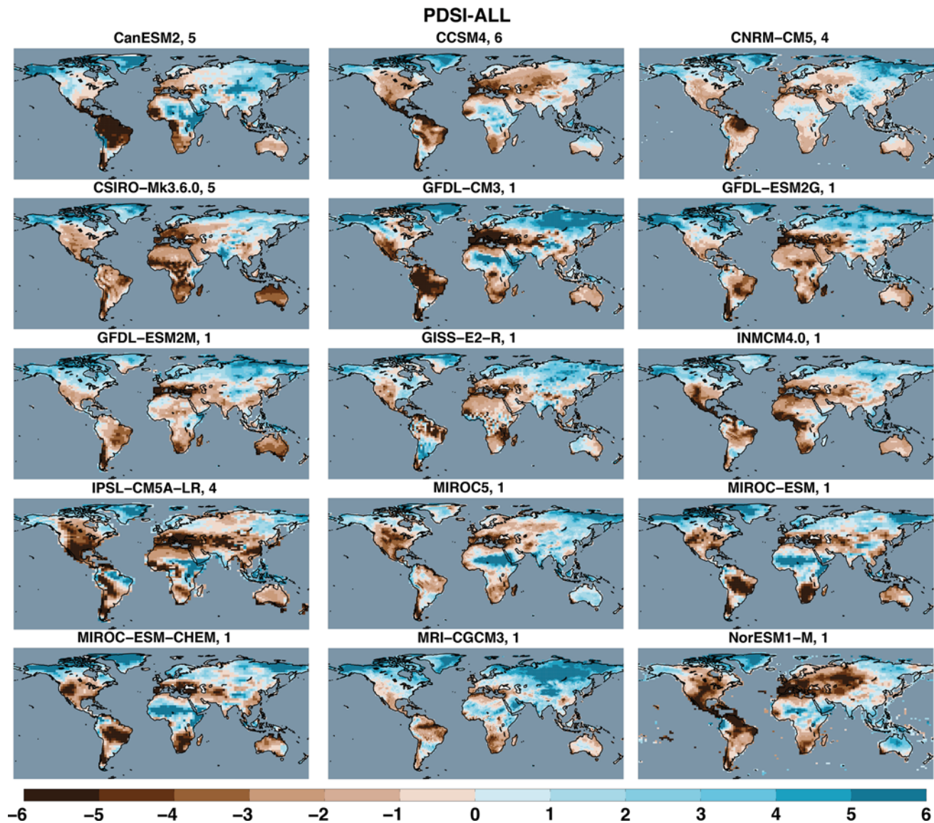
Fig. 5 Annual averaged PDSI-ALL from 2080–2099 for each model simulation under the RCP8.5 scenario. The number of ensemble members is listed in each panel title; for models with multiple ensemble members, the maps represent the ensemble average
