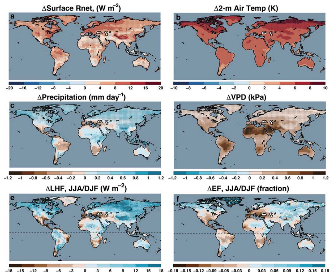
Fig. 4 Multi-model mean changes (2080–2099 minus 1931–1990) in a surface net radiation ( \text{W m}^{-2} ), b 2-m air temperature (K), c precipitation ( \text{mm day}^{-1} ), d vapor pressure deficit (kPa), e latent heat fluxes ( \text{W m}^{-2} ), and f evaporative fraction (fraction). a–d are annual averages. In e–f averages north of the equator (the dashed line)
