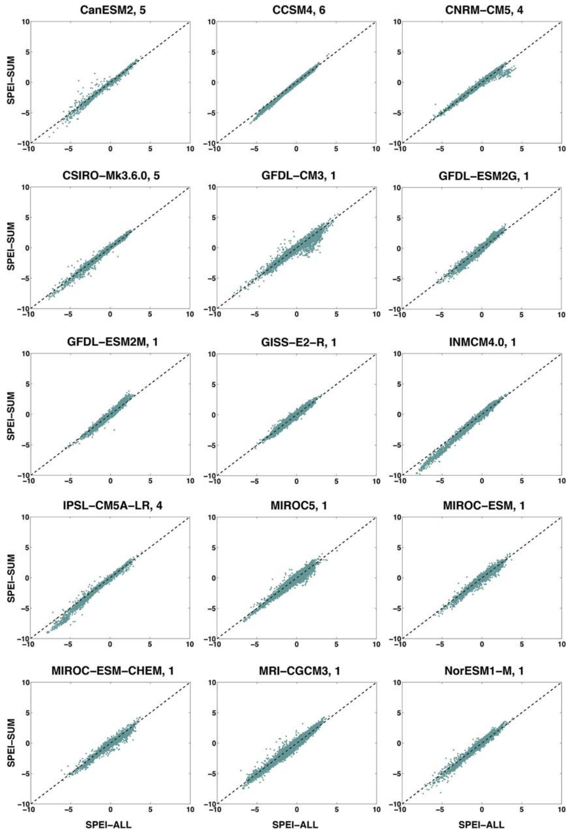
Fig. 3 Same as Fig. 2, but for the 12-month SPEI-ALL and SPEI-SUM calculations
