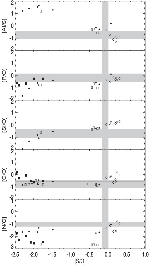
Fig. 11. Abundance ratios calculated from the stellar yields of Woosley & Weaver (1995). Yields are plotted for two mass ranges, 11–25 M_{\odot} (open symbols) and 30–40 M_{\odot} (filled symbols), and two metallicities, 0.1 Z_{\odot} (diamonds) and 0.01 Z_{\odot} (squares). The grey stripe shows the observed values. The horizontal black line shows the average ratio observed in the H II region of BCDs (Izotov et al. 1999).
