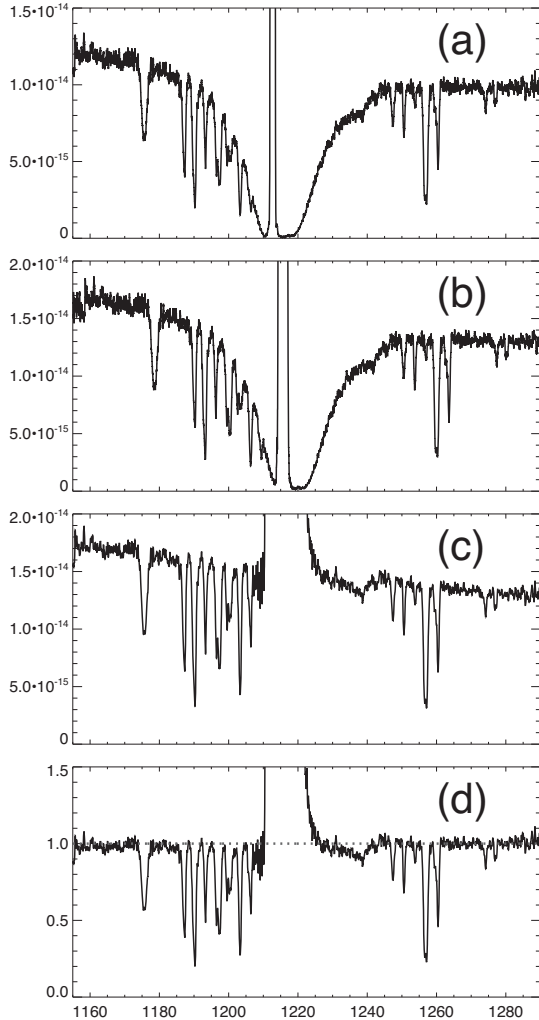
Fig. 2. Processing of the observed spectrum a) consists of correcting for reddening and for \text{Ly}\alpha absorption in the Milky Way and in the high-velocity cloud b) ; fitting and removing \text{Ly}\alpha from IZw 18 c) ; and normalizing the spectrum d) . The residual emission at \text{Ly}\alpha wavelength is due to geocoronal \text{H I} .
