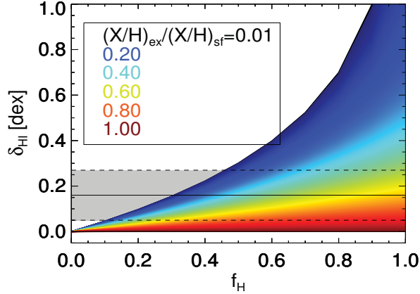
Fig. 12. Metal deficiency in the H I region \delta_{\text{H I}} , as a function of the fraction of hydrogen present in the HI-ex component defined as the extended H I component that may be less enriched in metals as compared to HI-sf (the H I component associated to the star-forming regions). We assume that the HI-sf component has the same metallicity as the H II region and calculate \delta_{\text{H I}} for several values of the sulfur abundance ratio between HI-ex and HI-sf . The horizontal dashed line and the grey stripe indicates illustrate the sulfur deficiency, \delta_{\text{H I}}(\text{S}) = 0.18 \pm 0.11 .
