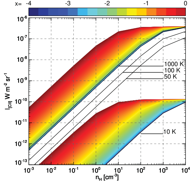
Fig. 6. The 157 \mu\text{m} cooling line intensity is calculated from Eq. (6) and is plotted as a function of the hydrogen number density and of the electron fraction ( x = n_e/n_H ). Note that the result should be scaled by the fraction of carbon in C^+ . The result should also be scaled by the carbon abundance with respect to the solar value and by the column density of hydrogen nuclei in units of 10^{21} \text{ cm}^{-2} . For temperatures 50 K and 100 K, only the curve for x = 0 is shown.
