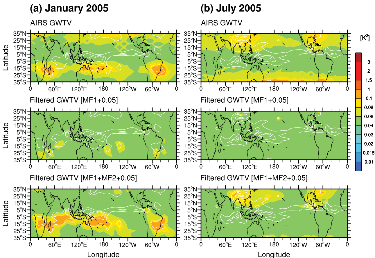
Figure 6. AIRS GWTVs and AIRS-filtered GWTVs from the parameterizations with the primary GW spectrum (MF1) and with both primary and secondary GW spectra (MF1+MF2) corrected by adding the background variance ( 0.05 \text{ K}^2 ) at z = 2.5 \text{ hPa} for (a) January and (b) July 2005. White lines denote the contours of the maximum NCEP DCH with 5, 8, and 10 \text{ K d}^{-1} in the troposphere.
