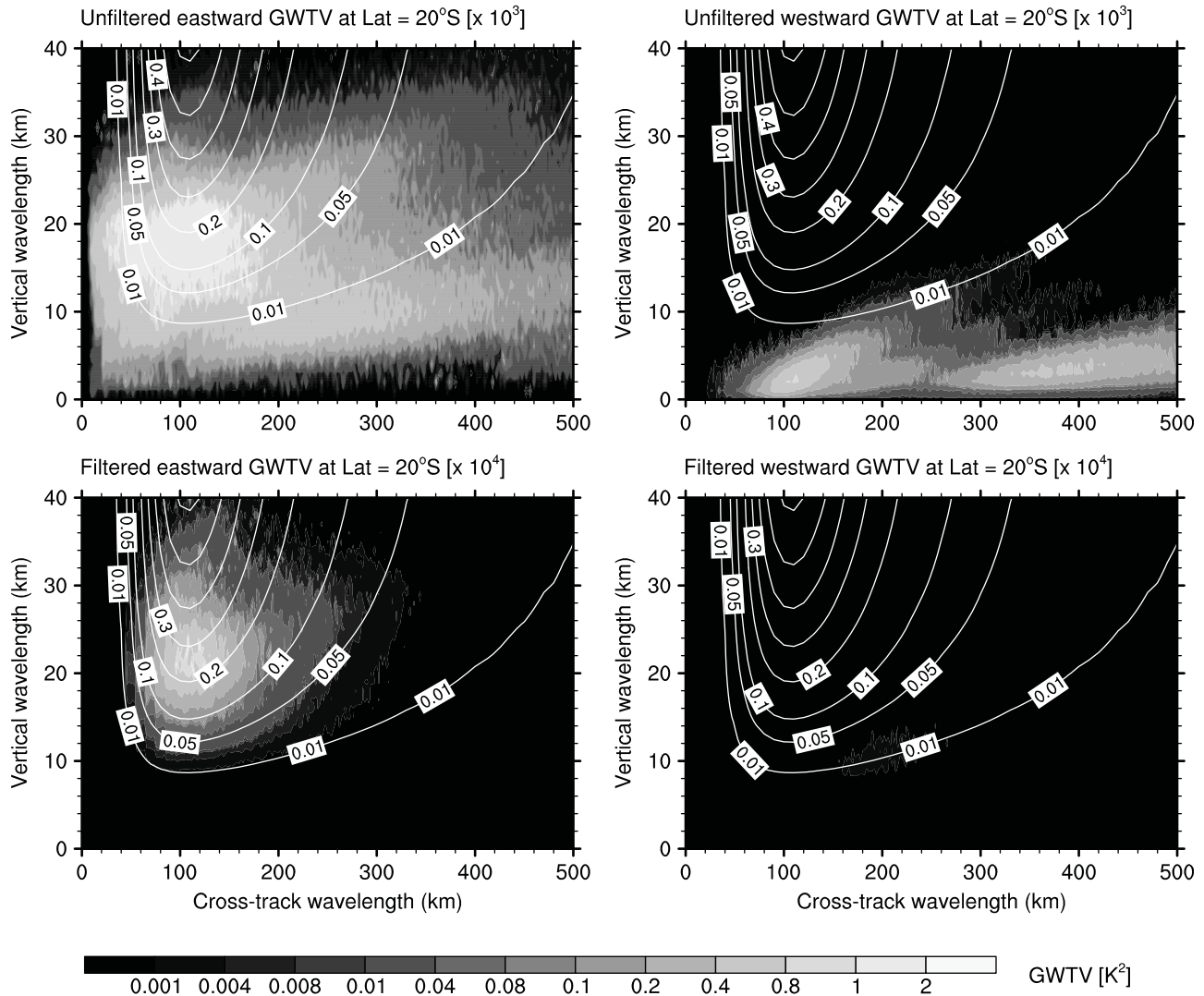
Figure 9. Unfiltered and AIRS-filtered summer subtropical (at 20°S) eastward and westward GWTVs at z = 2.5 hPa from the parameterization (shading) and the 2-D AIRS visibility (white lines) as a function of the cross-track and vertical wavelengths for January 2005. The unfiltered and AIRS-filtered GWTVs are multiplied by factors of 10^3 and 10^4 , respectively.
