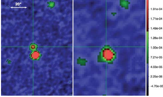
Fig. 9. PACS 100 ( left ) and 160 \mu\text{m} ( right ) images of HIP 82860. The crosshair denotes the position of the 100 \mu\text{m} flux peak. The angular scale is shown in the 100 \mu\text{m} image by a 20'' segment. Flux scale units are Jy/pixel. North is up and east to the left .
