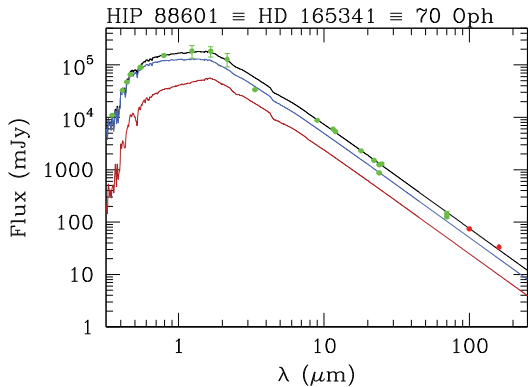
Fig. 5. Spectral energy distribution of the non-excess star HIP 88601. Plotted are optical, near-IR, WISE, and Spitzer MIPS (green symbols), as well as the PACS 100\ \mu\text{m} and 160\ \mu\text{m} (red symbols) fluxes. The photospheric fits of each individual component together with the added contribution of both stars (black) are shown as continuous lines.
