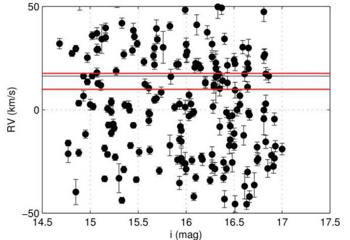
Figure 7. Radial velocity vs. SDSS i -band magnitude for the early-type stars selected from Knapp et al. (2007). The y-axis has been rescaled to show only the stars with RV between \pm 50 km s -1 . The mean RV of accepted members of Taurus (Luhman et al. 2009), 15.8 km s -1 , is shown with a black horizontal line. The neighboring red lines denote the region 9.8 \leq \text{RV} \leq 17.5 , our RV-member selection criterion. No concentration at the Taurus velocity is seen, and among those stars satisfying this RV criterion, most are too faint to be probable members of Taurus.
