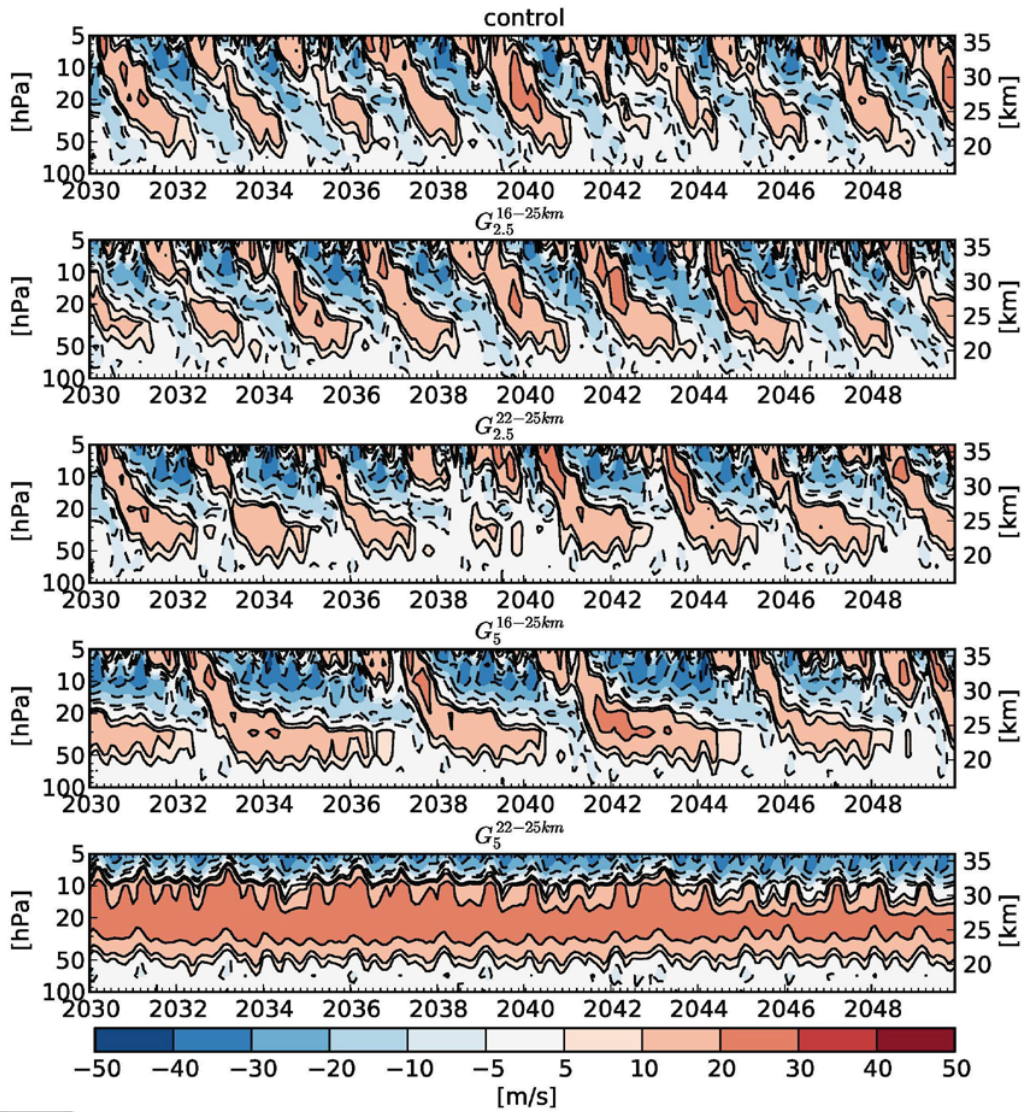
Fig.1: Vertical profiles of the zonal wind, zonally averaged between 2°S and 2°N in (from top to bottom) control run, G_{2.5}^{16-25km} , G_{2.5}^{22-25km} , G_5^{16-25km} , G_5^{22-25km} .
