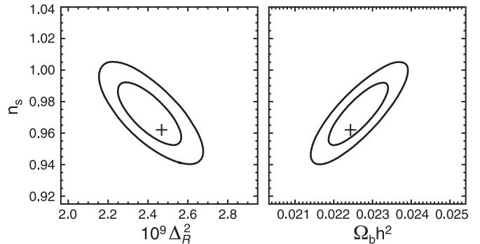
Figure 3. 68% and 95% CL regions for the \Lambda CDM parameters n_s , 10^9 \Delta_R^2 , and \Omega_b h^2 . There is a modest degeneracy between these three parameters in the six-parameter \Lambda CDM model, when fit to the nine-year WMAP data. The contours are derived from fits to the C^{-1} -weighted power spectrum, while the plus signs indicate the maximum likelihood point for the fit to the MASTER power spectrum. As shown in Figure 2, the two model produce nearly identical spectra.
