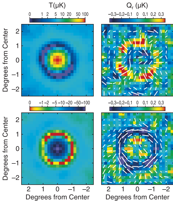
Figure 12. Co-added maps of temperature, T , and polarization, Q_r , smoothed to a common resolution of 0^\circ.5 , and stacked by the location of temperature extrema. (The polarization maps were not smoothed for the analysis, however.) Top left: the average temperature hot spot. Top right: the rotated polarization map, Q_r , stacked around temperature hot spots. Bottom left: the average temperature cold spot. Bottom right: the rotated polarization map, Q_r , stacked around temperature cold spots. The polarization images are color-coded so that the red ( Q_r > 0 ) shows the radial polarization pattern, while blue ( Q_r < 0 ) shows the tangential polarization pattern. The lines indicate polarization direction. These images are a striking illustration of BAO in the early plasma, and phase coherence in their initial conditions.
